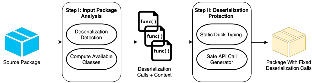
Fig. 4: Overview of QUACK’s analysis process. First, QUACK conducts the analysis step to identify calls to deserialization APIs, determine the set of available classes at the call site, and infer the intended set of allowed classes for the deserialized object. Then, it protects the application by rewriting the vulnerable call sites to restrict the allowed classes and produce safe deserialization calls.
