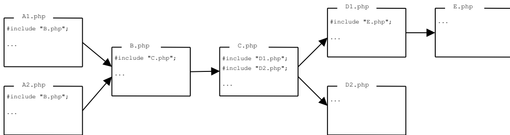
Fig. 6: QUACK constructs and traverses the class-def-graph (CDG) to identify the available classes at each program location.
