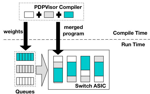
Figure 3. PDPVisor: overview.
