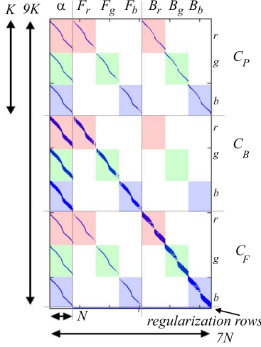
Figure 6: Sparsity structure of J . Background colors in the diagram represent the color channel corresponding to each term. Dark blue marks non-zero elements.
