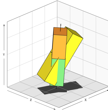
(c) 30^\circ @ b = 1000 \text{ s/mm}^2 , \sigma = 14.5 .
