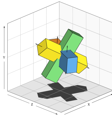
(e) 3X @ b = 1000 \text{ s/mm}^2 , \sigma = 14.5 .
