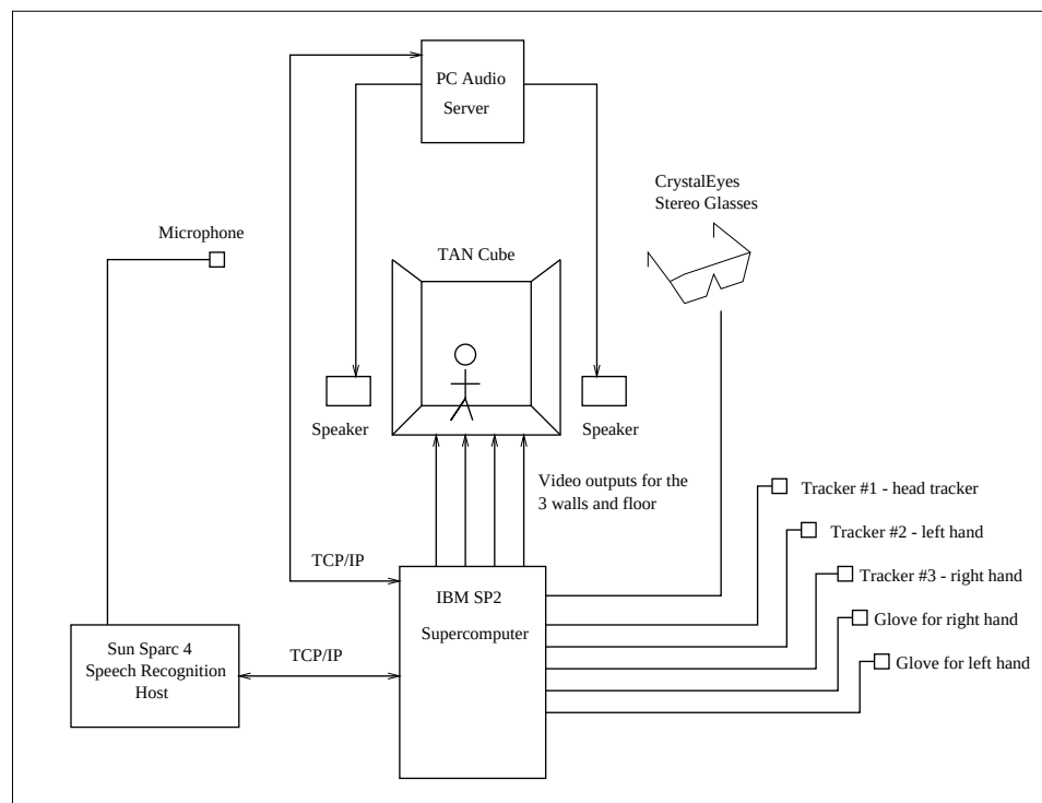
Figure 5.3: The various components that make up the surround screen hardware configuration.
