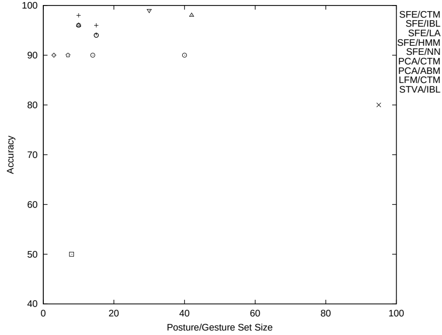
Figure C.1: A graph showing posture and gesture set sizes and accuracies for different feature extraction-classification combinations. The key to the abbreviations is found in Table C.1.
