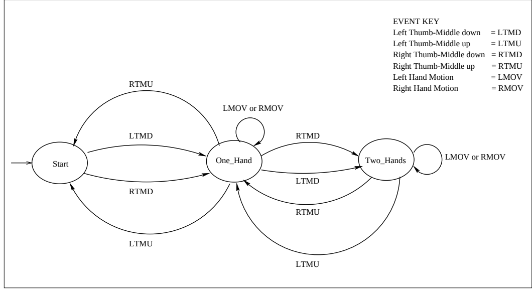
Figure 5.6: An example finite state machine created within our multimodal interface framework. The arcs are event transitions which send the interaction technique into a particular state. In this case, there are three states and a total of 10 event transitions.
