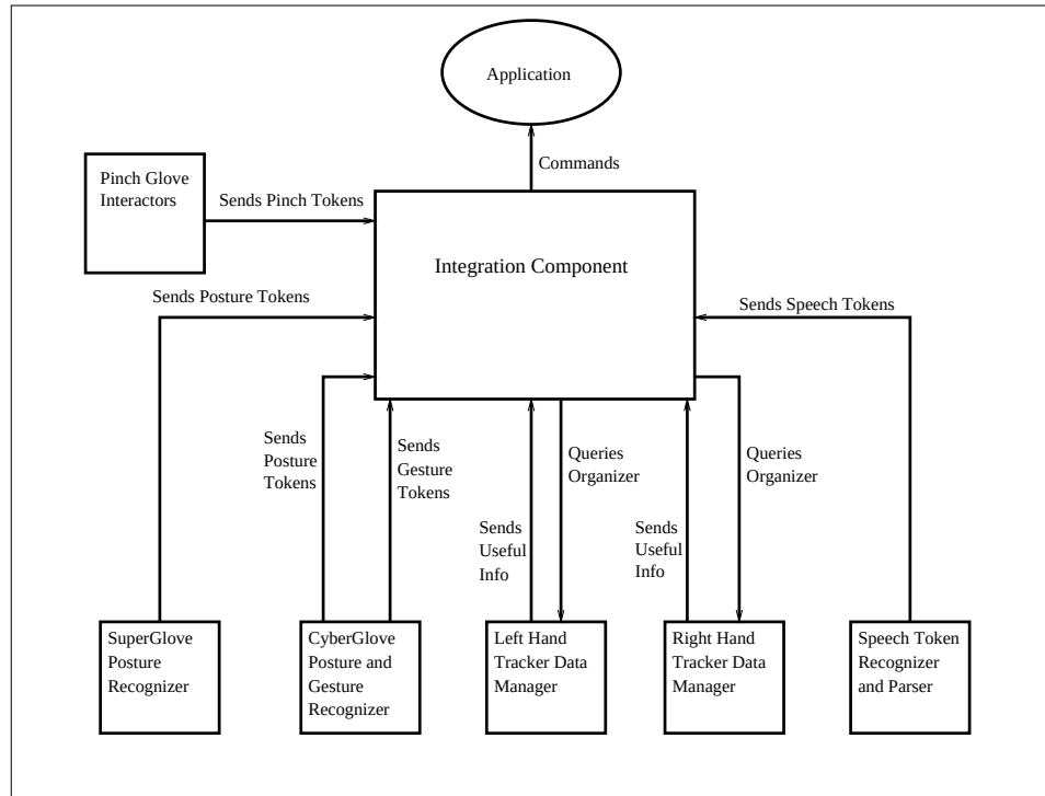
Figure 5.5: The components that make up our multimodal interface framework. Arrow indicate direction of data flow.
