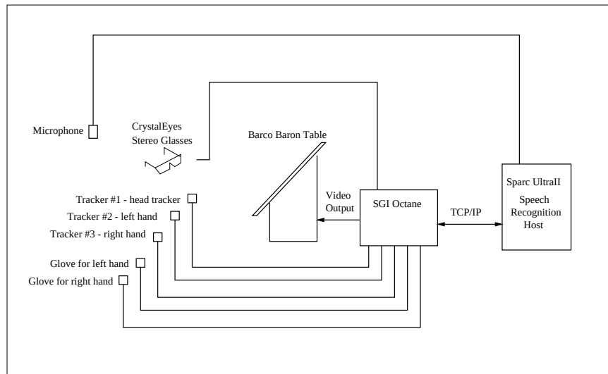
Figure 5.1: The various components that make up the rear-projected display table configuration.
