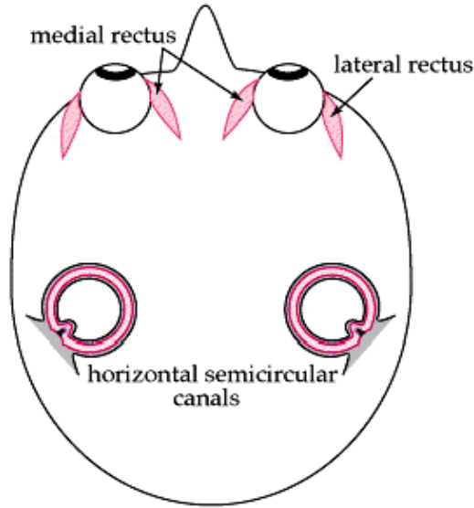
Figure 3: A top down view of a person's head showing the horizontal semicircular canals and the medial and lateral rectus. The figure is adapted from[22].
