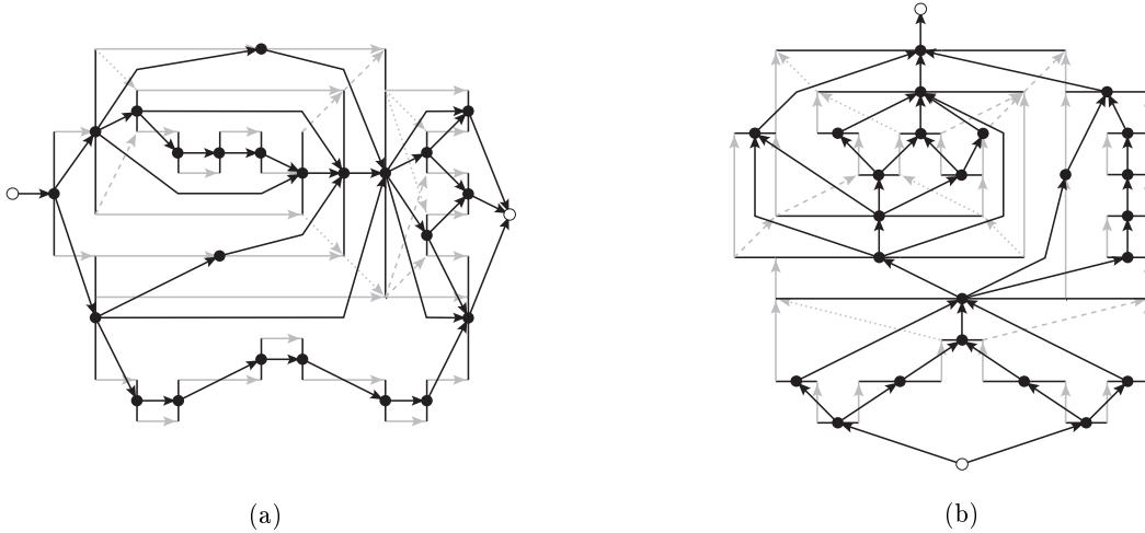
Figure 19: (a) D_x . (b) D_y . Both graphs are obtained from graphs H_x and H_y shown in Fig. 10.
