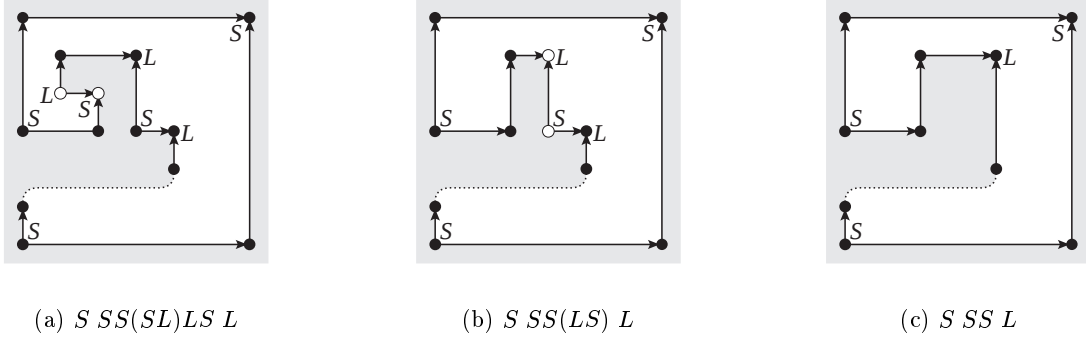
Figure 7: Collapsing a sequence of switches. In each step, the switches being collapsed are represented as white circles, and the SL or LS pair of labels being removed is shown in parentheses.
