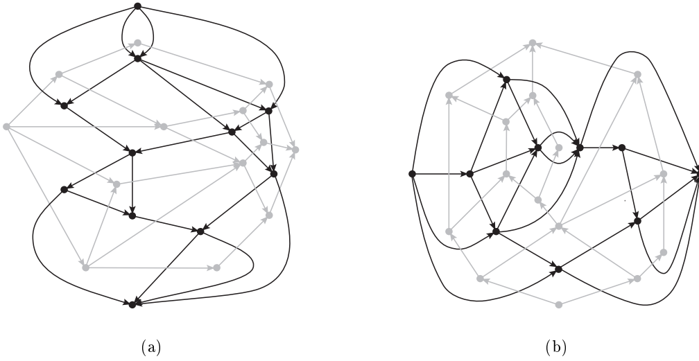
Figure 20: (a) N_x . (b) N_y . The corresponding planar st -digraphs D_x and D_y are represented in grey.
