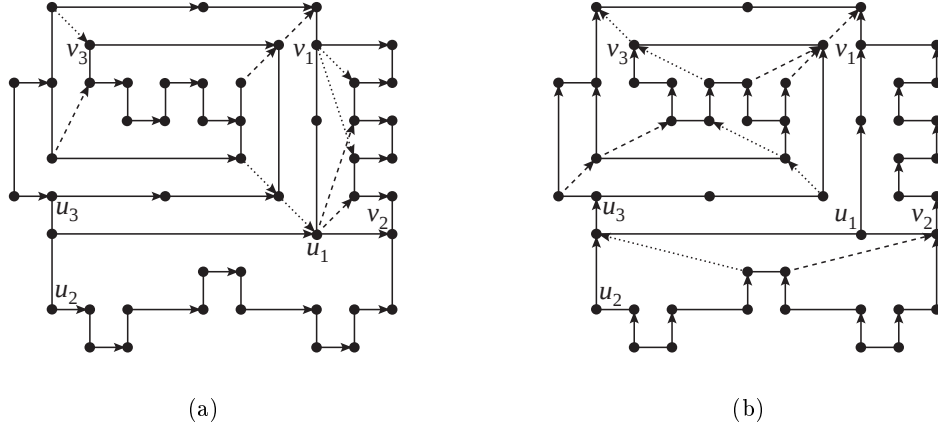
Figure 10: (a) H_x . (b) H_y . Both graphs are obtained using the complete saturators shown in Fig. 9.
