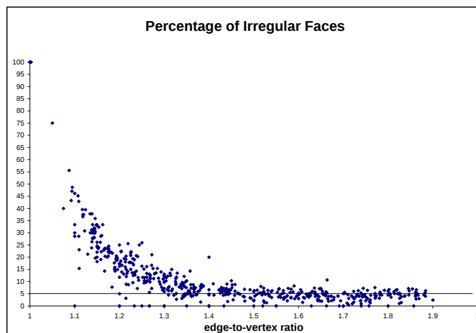
Figure 21: The percentage of non-regular faces with respect to the edge-to-vertex ratio.
