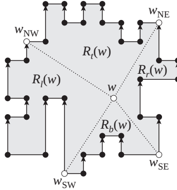
Figure 15: The four regions of vertex w .
