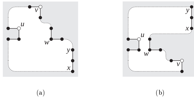
Figure 16: The two cases in the proof of Lemma 11.
