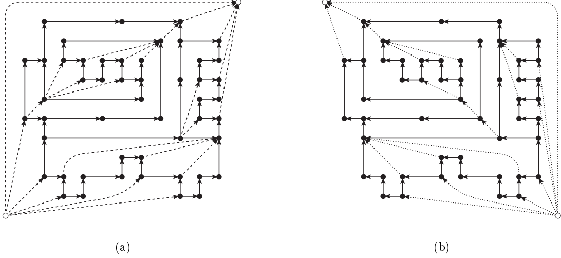
Figure 9: (a) G_r (edges represented as solid segments) and a complete saturator (edges represented as dashed segments). (b) G_\ell (edges represented as solid segments) and a complete saturator (edges represented as dotted segments).
