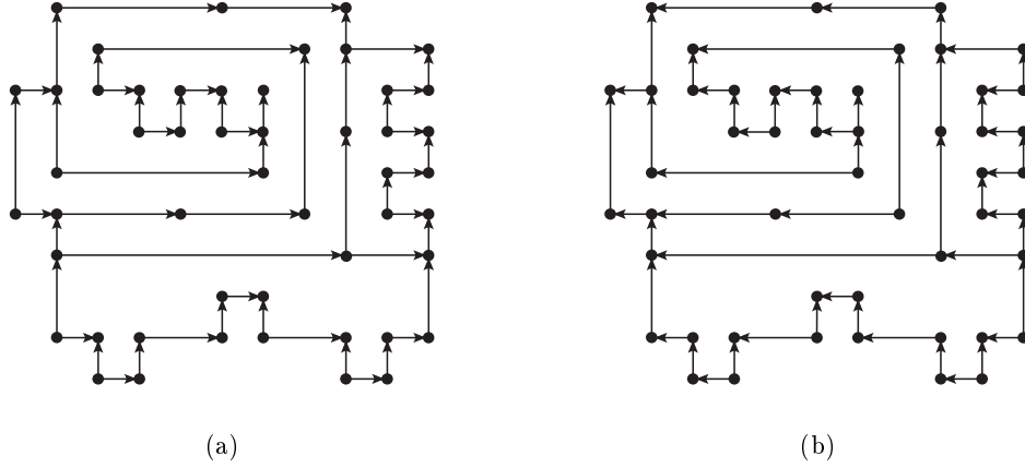
Figure 4: Two orientations of the same orthogonal representation. (a) H_r . (b) H_\ell .
