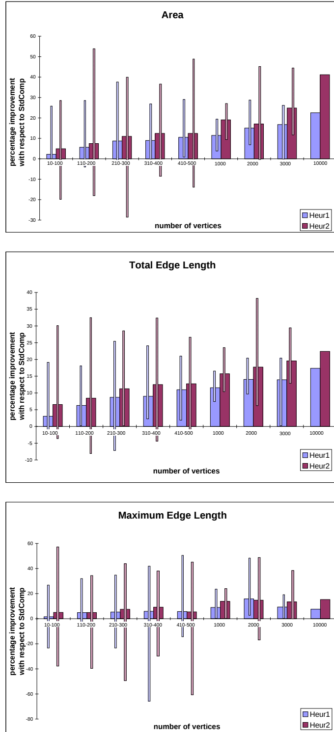
Figure 22: The average percentage improvement in area, total edge length, and maximum edge length of Heur1 and Heur2 with respect to StdComp. The narrow columns show the minimum and maximum improvement.
