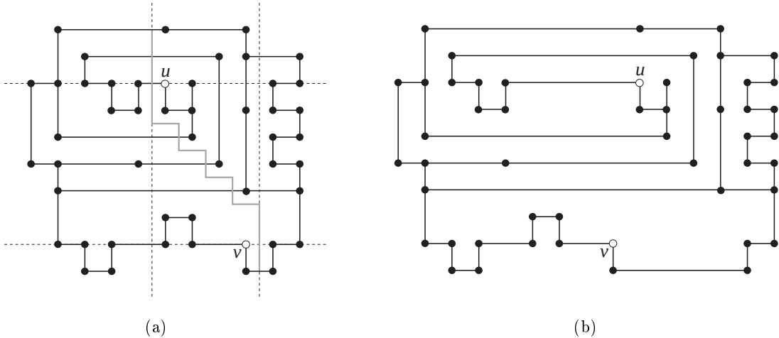
Figure 18: (a) A planar orthogonal drawing \Gamma with the extended moving-line for vertices u and v . (b) The stretched version of \Gamma .
