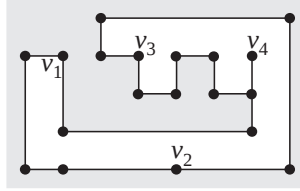
Figure 3: A face of an orthogonal representation. The grey portion represents the rest of the graph.
