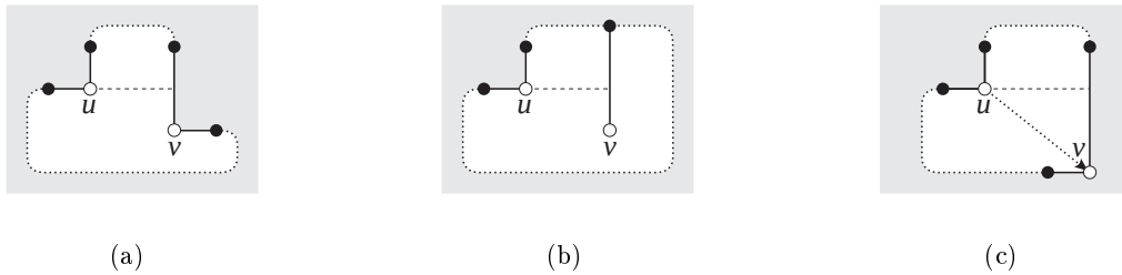
Figure 17: Three cases in the proof of Lemma 12. The horizontal segment connecting u to mvc_2 is represented as a dashed segment.
