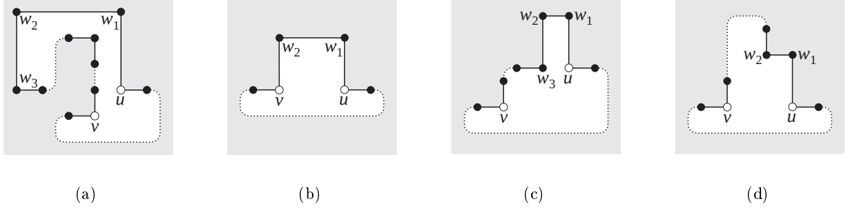
Figure 14: Four cases in the proof of Lemma 9.
