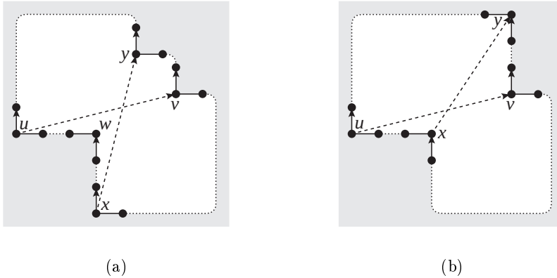
Figure 12: Impossible cases of crossing saturating edges in H_y .
