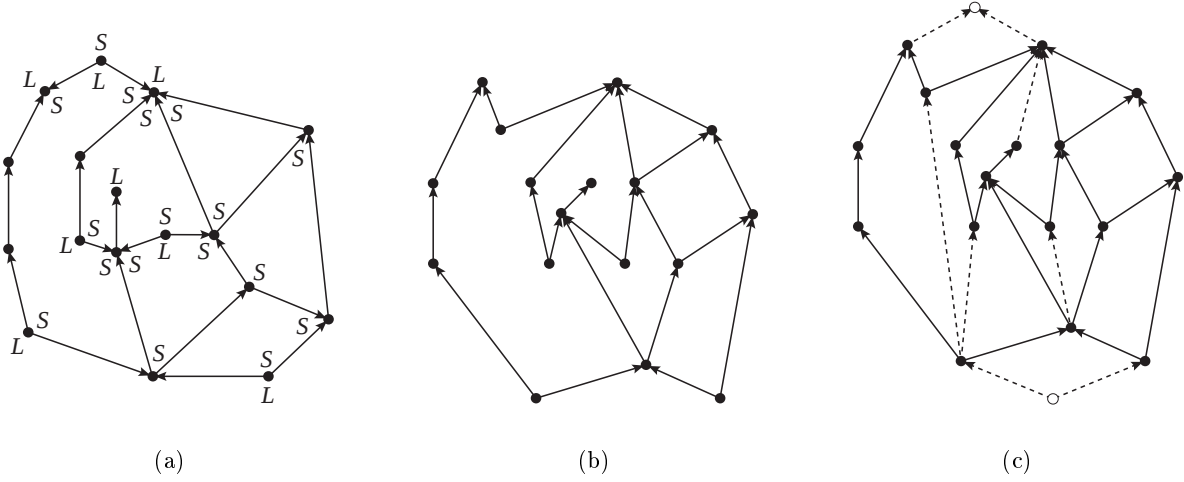
Figure 2: (a) A bimodal embedded planar digraph G with an upward consistent labeling of its faces. (b) An upward planar drawing of G corresponding to the upward consistent labeling in (a). (c) A complete saturator of G ; s and t are represented as white circles, and saturating edges are represented as dashed segments.
