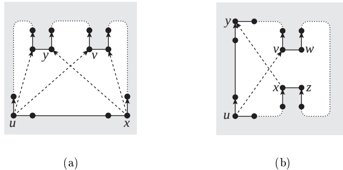
Figure 13: Crossing saturating edges of H_y .
