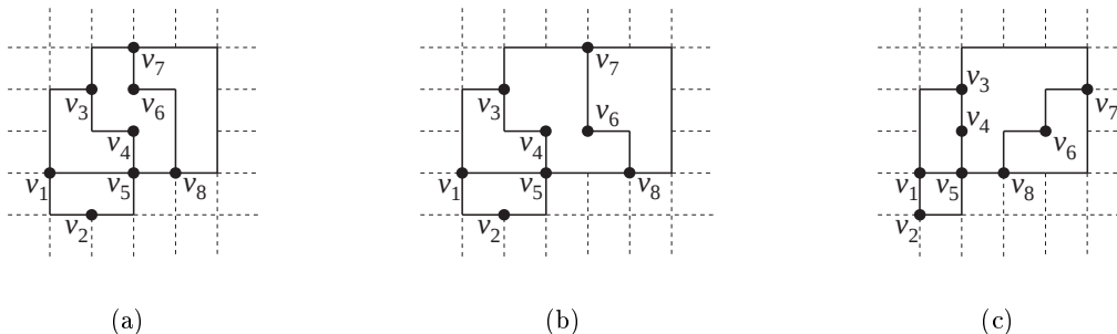
Figure 1: Three planar orthogonal drawings of a graph. Two drawings of the same orthogonal representation are shown in (a) and (b), while a drawing of a different orthogonal representation is shown in (c). The drawing in (a) has optimal area among all planar drawings of that orthogonal representation.
