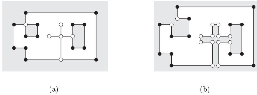
Figure 5: (a) A face f of an orthogonal representation. The vertices affected by the expansion are represented as white circles. (b) The expanded face corresponding to f .
