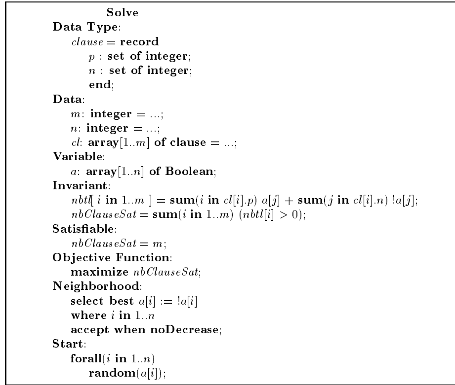
Figure 3: A Simple Model of GSAT
