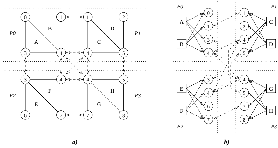
Figure 5: A square mesh partitioned by elements between four processors (a) and its internal representation using remote references (b).
