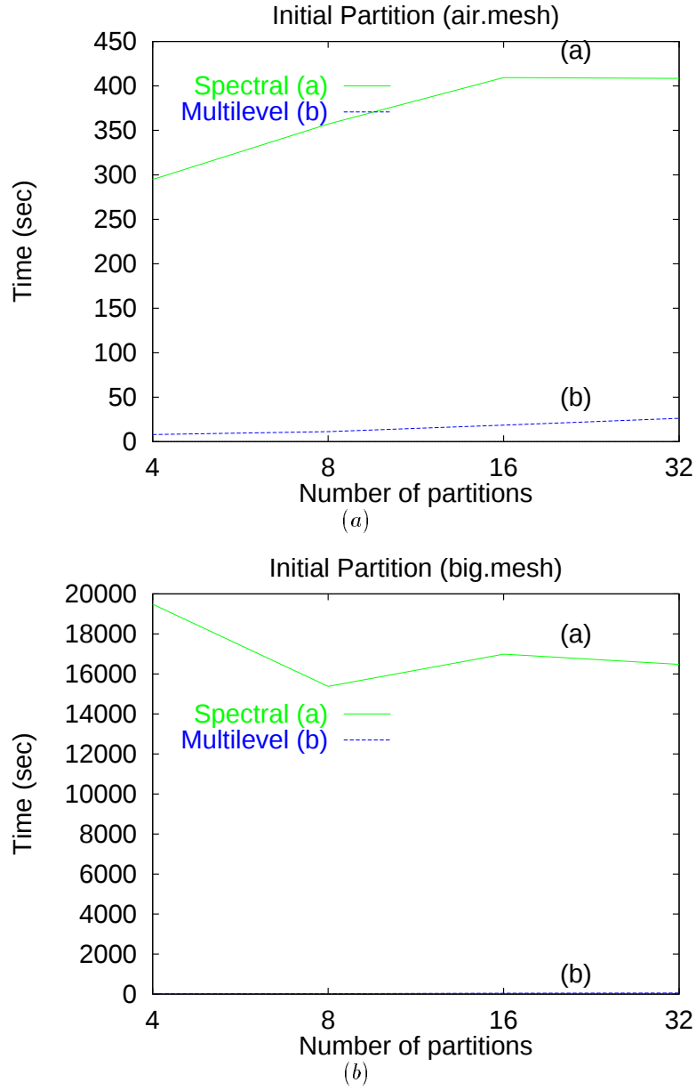
Figure 36: Partition of the initial mesh using Chaco . Time spent to compute 4, 8, 16 and 32 partitions of (a) air.mesh and (b) big.mesh .
