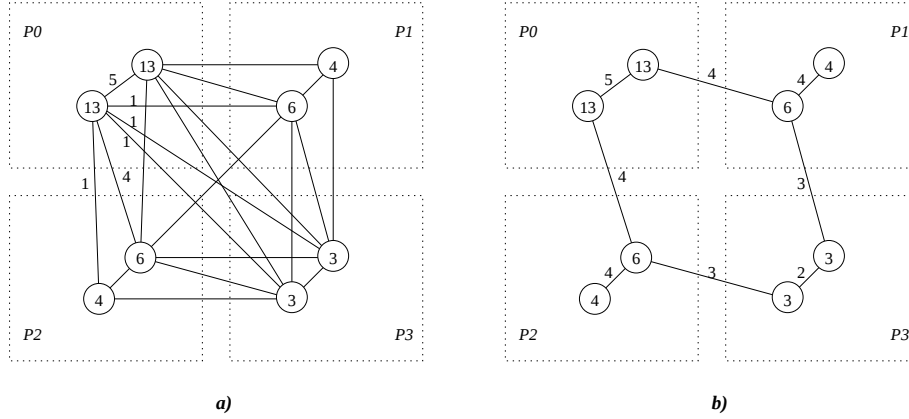
Figure 18: The parallel Nested Repartitioning algorithm.
