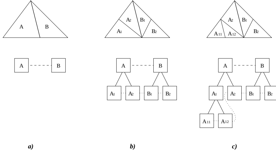
Figure 4: Multilevel refinement. Initially elements E_a and E_b in (a) are selected for refinement. Both elements are refined and replaced by their children (b). In (c) the element E_{a_1} is further refined. Under the meshes we show the corresponding mesh hierarchy.
