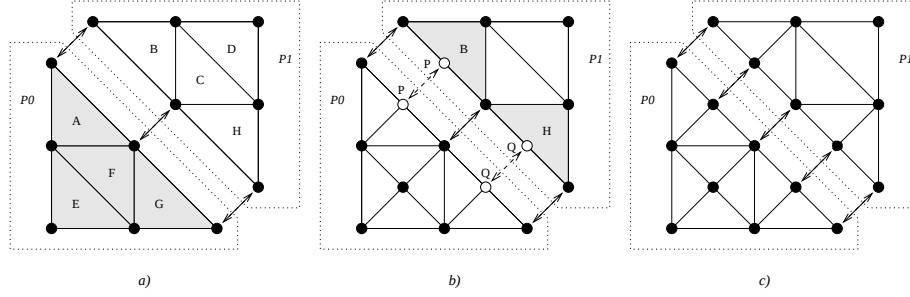
Figure 8: Propagation of refinement to adjacent processors. In (a) the elements E_a, E_e, E_f and E_g are selected for refinement. The refinement of these elements creates two nodes, V_p and V_q , in the boundary between P_0 and P_1 . P_1 creates its local copies V_p^1 and V_q^1 and selects the nonconforming elements E_b and E_h for refinement (b). (c) shows the resulting mesh.
