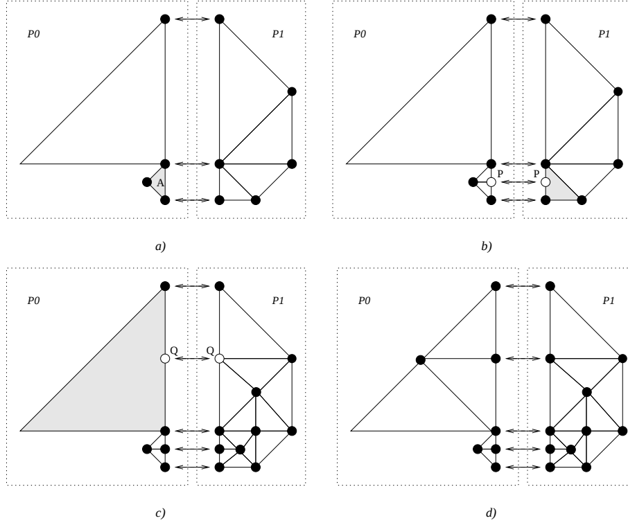
Figure 12: A propagation cycle. P_0 has initially one element marked for refinement (a). The refinement propagates to P_1 (b) and then comes back to P_0 (c). (d) shows the final mesh.
