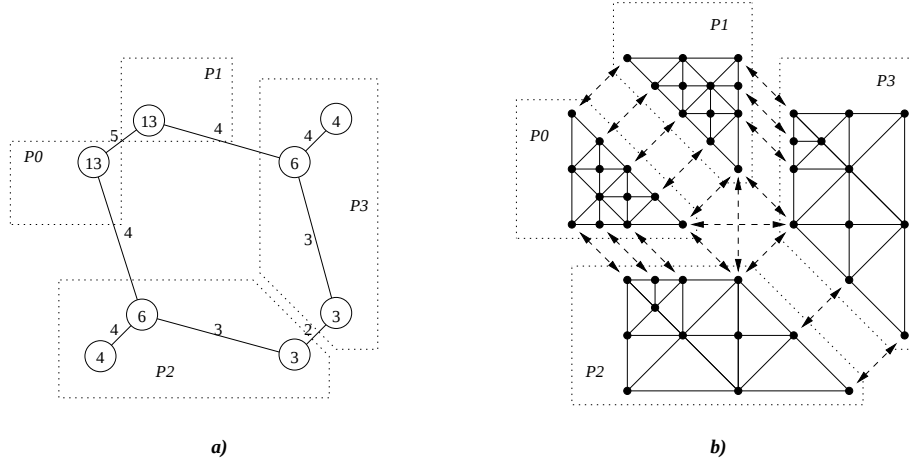
Figure 20: The Parallel Nested Repartitioning algorithm. (a) shows the partition \Pi of M using the PNR algorithm. Finally we use the migration algorithm to migrate elements and nodes to their destination processors. (b) shows the resulting mesh.
