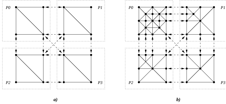
Figure 17: The Parallel Nested Repartitioning algorithm. (a) shows the initial mesh M_0 and (b) shows the mesh M_t at the beginning of the partitioning phase.
