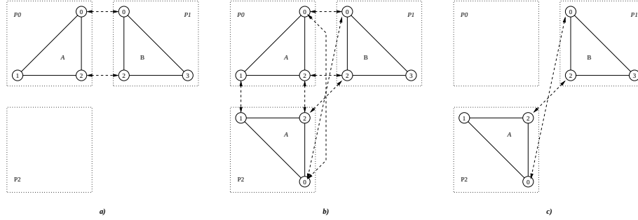
Figure 21: A migration example. (a) shows the initial mesh. The goal is to move E_a from P_0 to P_2 . We first copy E_a to P_2 (b) and then we delete the element E_a in P_0 (c).
