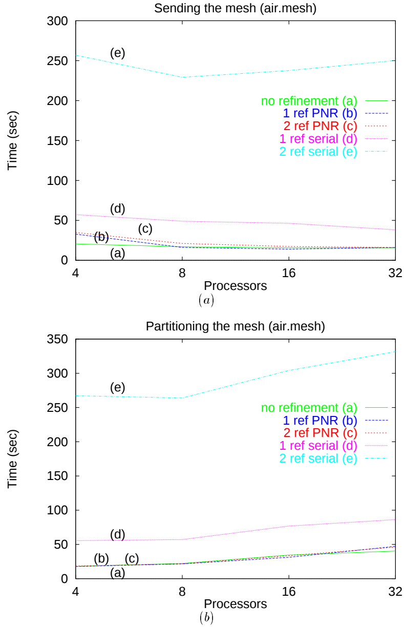
Figure 43: Partitioning of the mesh after none, one and two refinements using the PNR algorithm and the serial Multilevel Bisection algorithm. (a) shows the time spent on sending the mesh to one processor. (b) shows the time spent by P_0 to partition the graph.
