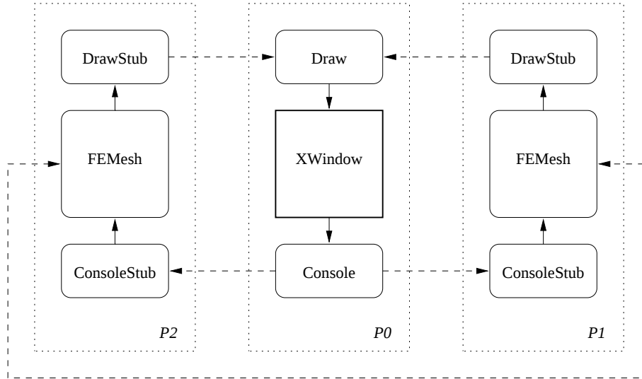
Figure 31: Implementation of the distributed input/output.
