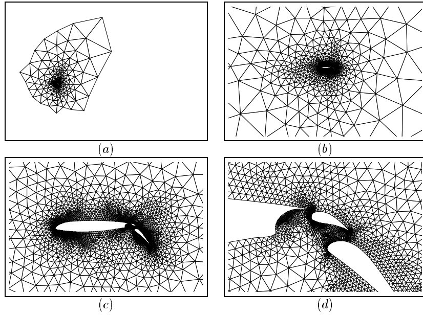
Figure 34: The air.mesh is a 2D finite element grid of a complex airfoil with triangular elements. It consists of 9000 elements and 4720 nodes. This mesh is provided with the Chaco program.
