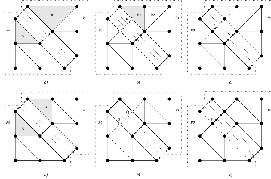
Figure 9: Refinement of adjacent elements located in different processors. In the top row two elements are selected for refinement (a). The refinement of E_a creates the shared node V_p (b). We then select E_{b_1} for further refinement (rather than E_b ) (c). The bottom row shows another example (a) where two processors create shared nodes in the same position (b). In (c) we detect this problem and update the references.
