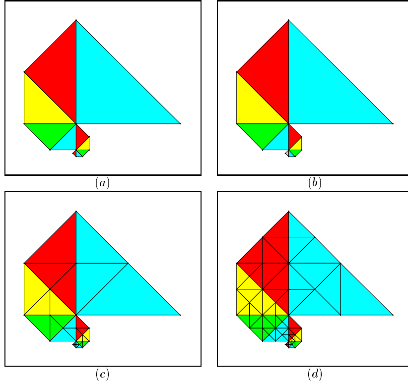
Figure 15: Propagation of the refinement. In (a) we show an arbitrary mesh distributed in 4 processors. The refinement of an element (b) causes the refinement to come back to the processor (c). If we repeat this operation we obtain the mesh in (d).
