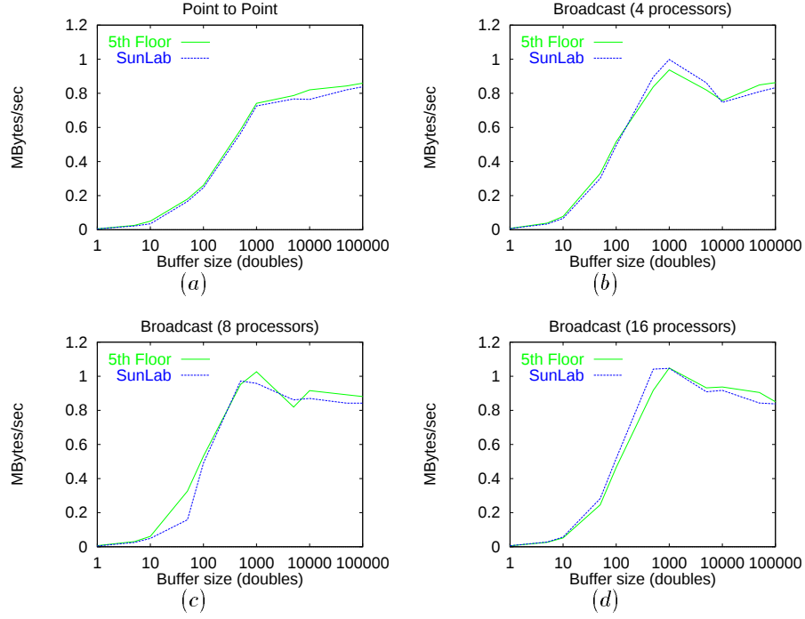
Figure 32: Comparison of the performance of the network between machines in the 5th floor and machines in the SunLab. (a) shows the performance of a ping application where a source processor sends a message to a destination processor and then waits for a response. This example is used to measure the latency of the network. Only when the messages are around 8K (1000 doubles) we do obtain full speed. (b), (c) and (d) show the performance of a broadcast example where a source processor sends an individual message to every other processor and waits for a response from all of them.
