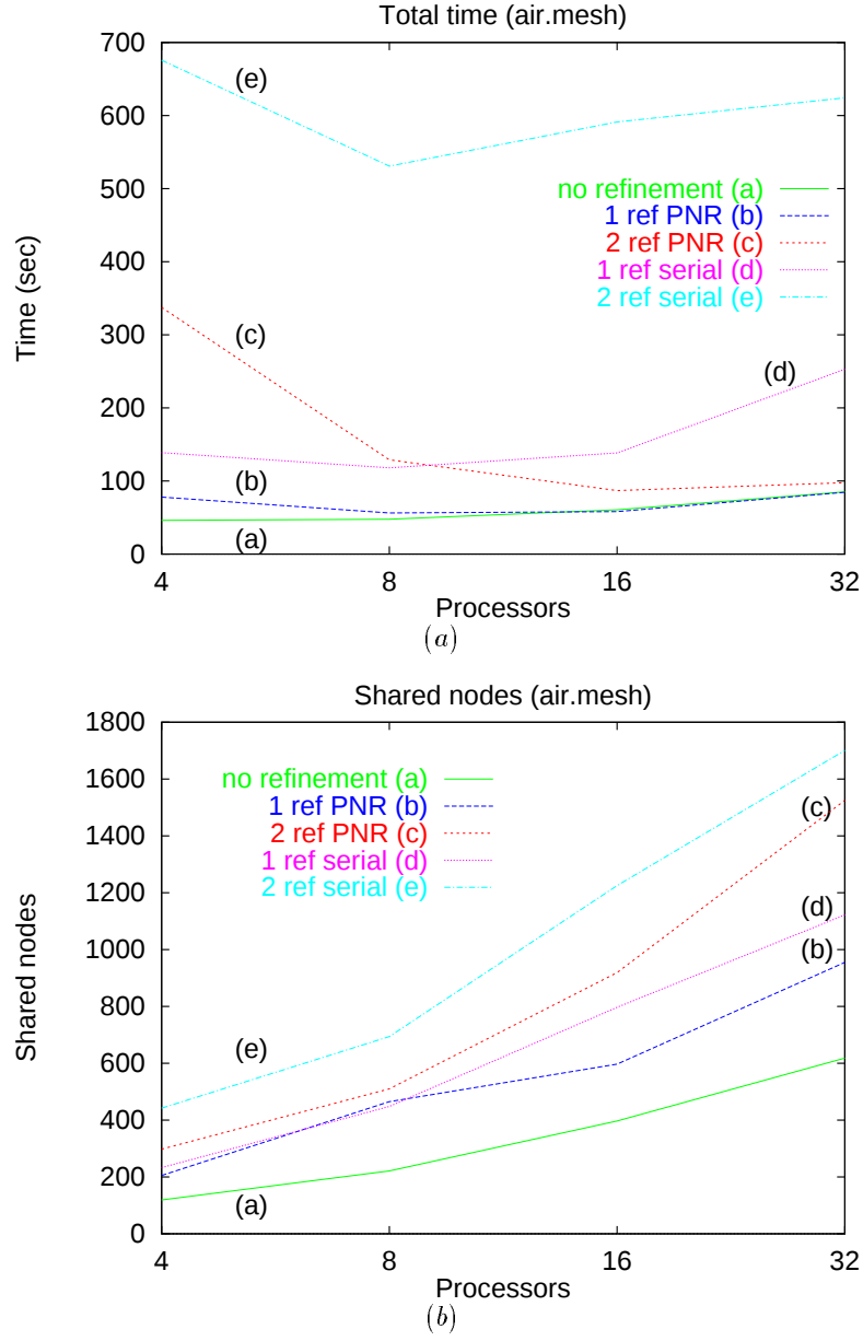
Figure 45: Partitioning of the mesh after none, one and two refinements using the PNR algorithm and the serial Multilevel Bisection algorithm. (a) is the total time. The number of shared nodes is shown in (b).
