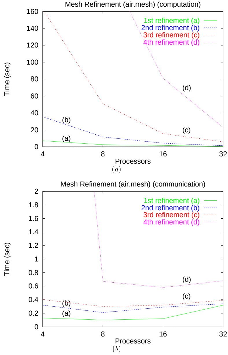
Figure 38: Successive refinements of the mesh. In (a) we show time spent in the serial part of the algorithm while in (b) we show the time spent on communication.
