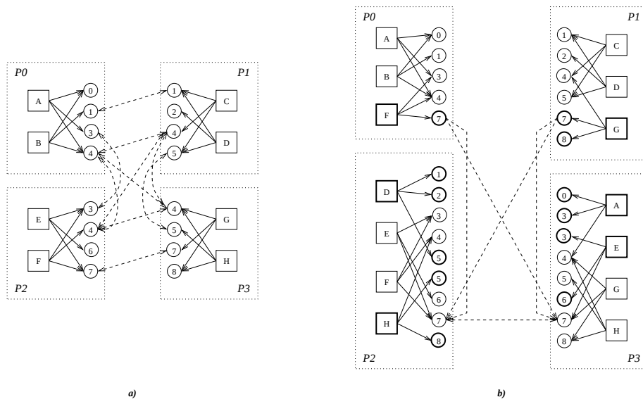
Figure 23: A migration example: internal representation of the mesh at the beginning of the migration (a) and after copying the elements to the destination processors (b).
