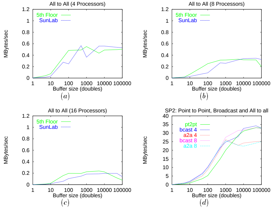
Figure 33: Comparison of the performance of the network between machines in the 5th floor and machines in the SunLab and the performance of the same applications run on the SP2. (a), (b), (c) show the performance of an all to all communication example where each processor sends a message to each other. These example are a measure of the contention on the network. (d) is the result of running the same tests on the SP2.
