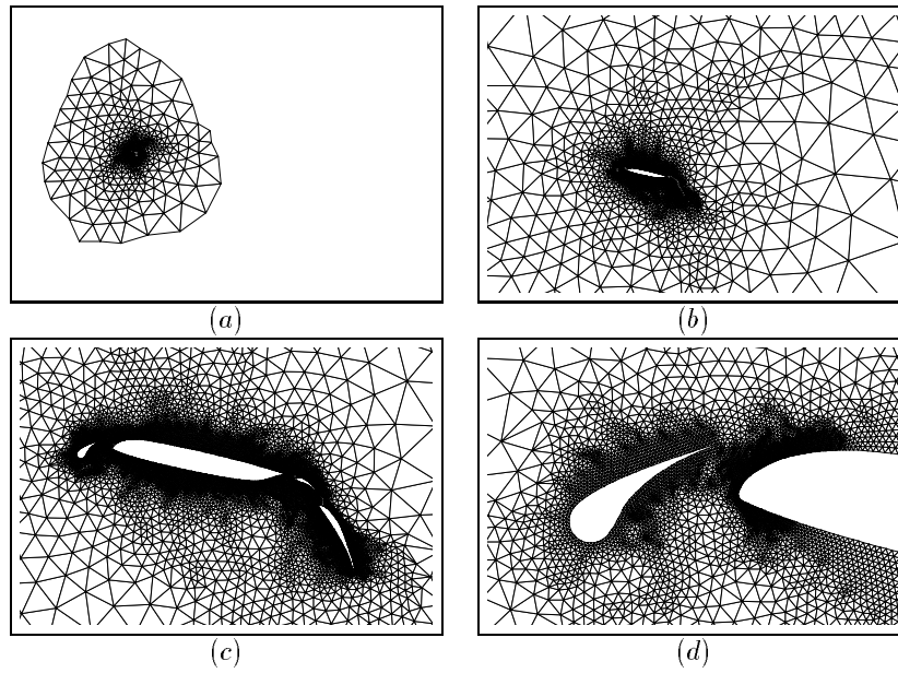
Figure 35: The big.mesh is a 2D finite element mesh of a complex airfoil. It consists of 30269 elements and 15606 nodes. It is obtained from riacs.edu in the directory “ pub/grids/big.* ”.
