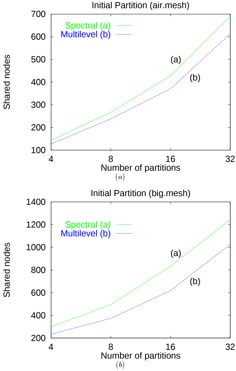
Figure 37: Partition of the initial mesh using Chaco . Number of shared of nodes after computing the partitions of (a) air.mesh and (b) big.mesh .
