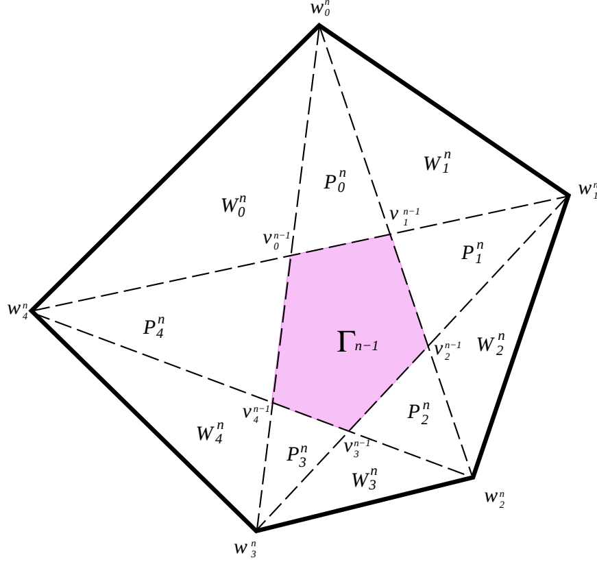
Figure 8: Extruded pentagon of F_5^{n-1} .
