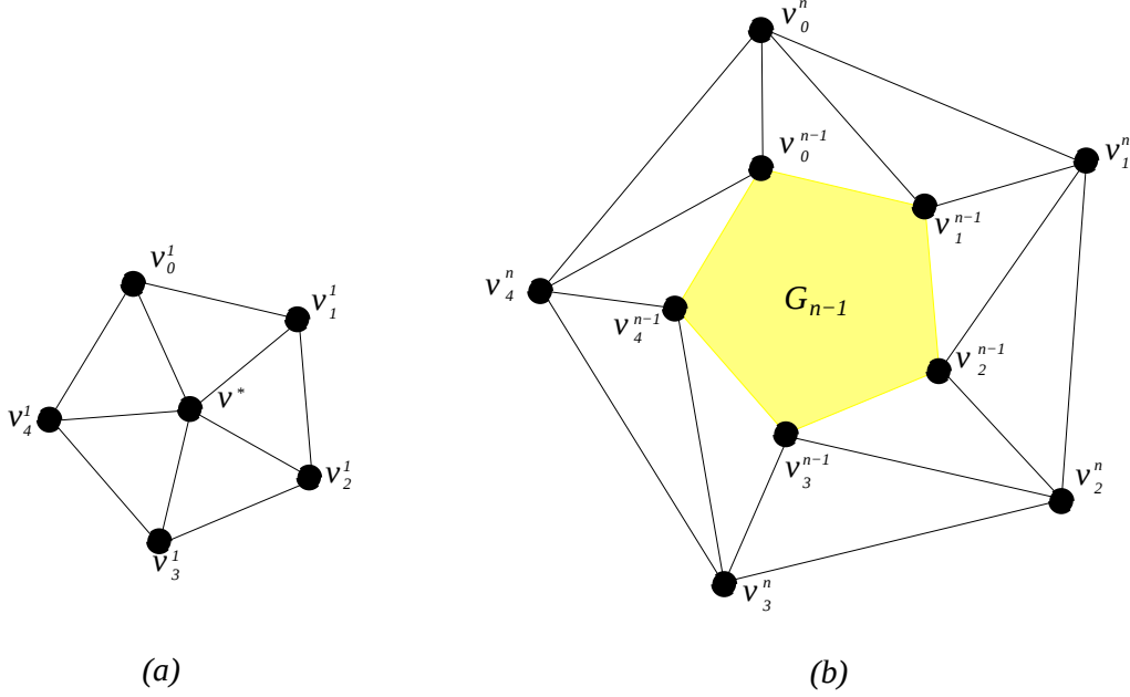
Figure 3: A class of graphs that require exponential area.
