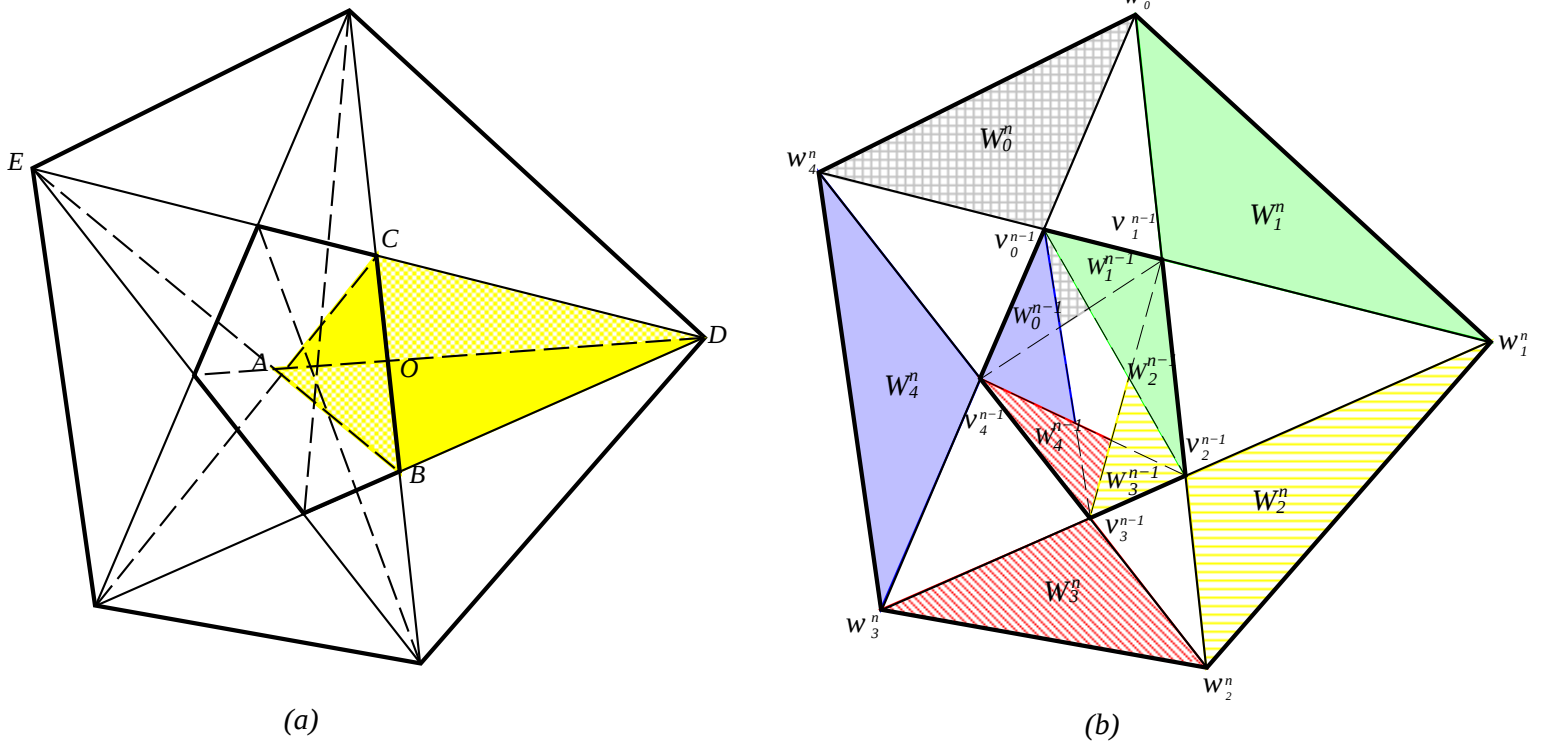
Figure 9: Covering of \Gamma_{n-1} .
