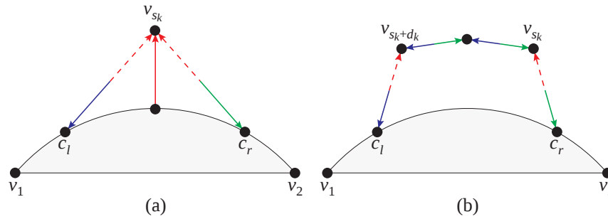
Figure 3: The coloring of the edges in the construction of a realizer. (a) V_k = \{v_{s_k}\} . (b) V_k = \{v_{s_k}, \dots, v_{s_k+d_k}\} .
