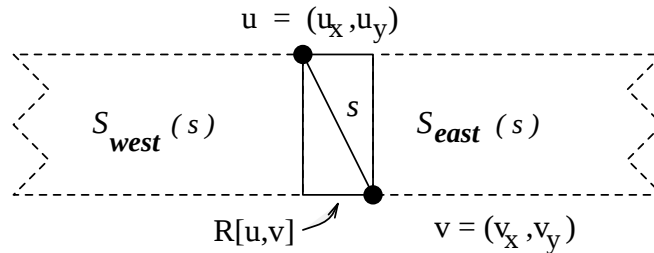
Figure 11: Strips for segment s .
