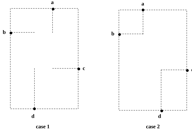
Figure 10: Figure for Theorem 4.4.
