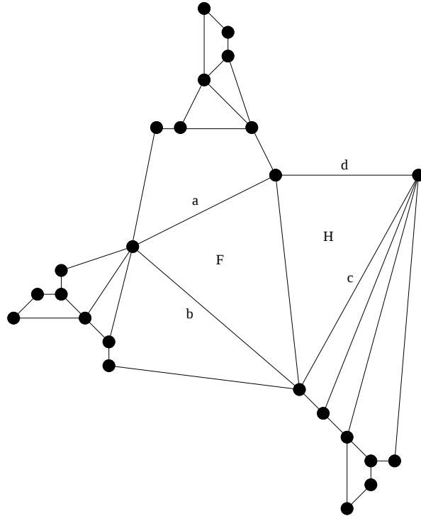
Figure 19: A closed rectangle of influence drawing of G .
