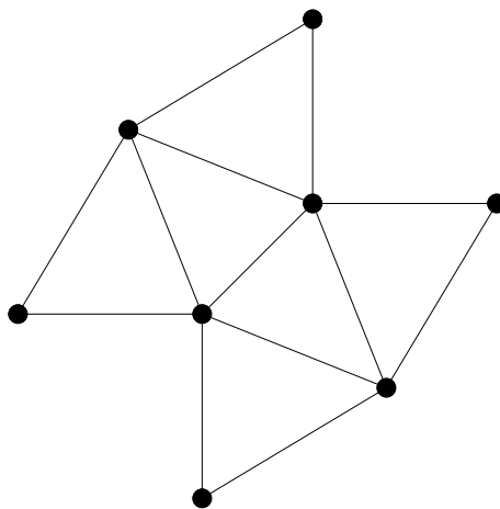
Figure 20: A closed rectangle of influence drawing of an outerplanar graph whose dual tree has four leaves.
