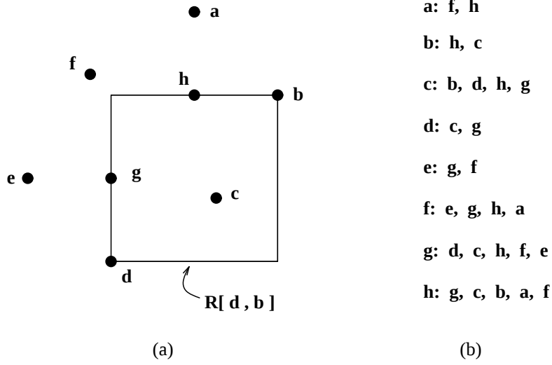
Figure 3: (a) A set of points P , and (b) the graph RIG[P] .
