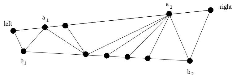
Figure 6: How to draw a maximal outerplanar open RID graph.
