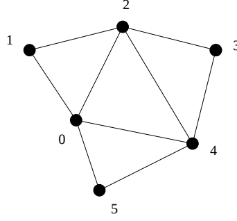
Figure 7: A non-open RID outerplanar graph.
