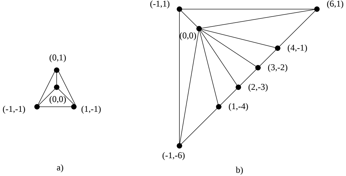
Figure 4: Illustration for Theorem 4.1 for a) n = 4 and b) n = 8 .
