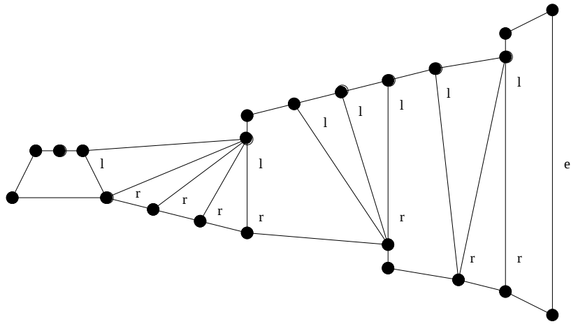
Figure 16: Closed rectangle of influence drawing of the graph in Figure 12.
