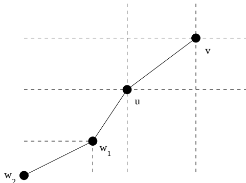
Figure 5: Illustration for Theorem 4.2.
