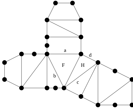
Figure 18: An outerplanar graph G whose dual tree has three leaves.
