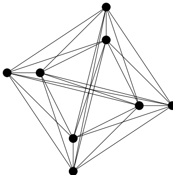
Figure 9: An open rectangle of influence drawing of K_8 .
