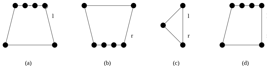
Figure 13: Drawings for face F_0 .
