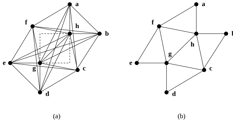
Figure 1: Examples of rectangle of influence drawings for (a) the closed model and (b) the open model.
