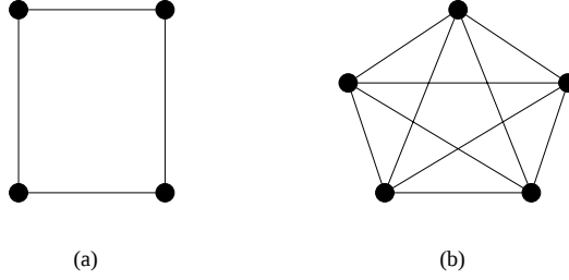
Figure 2: Examples of rectangle of influence drawings for (a) a 4-cycle and (b) K_5 .
