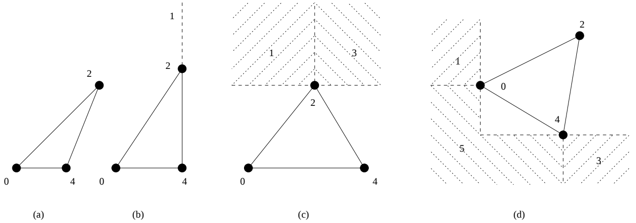
Figure 8: Illustration for Lemma 4.2.
