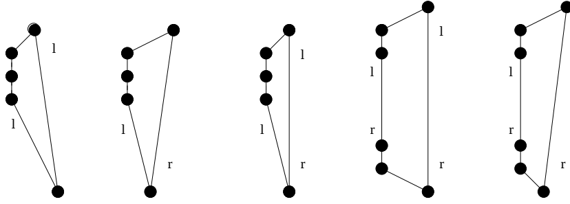
Figure 14: Drawings for face F_i for 0 < i < t .
