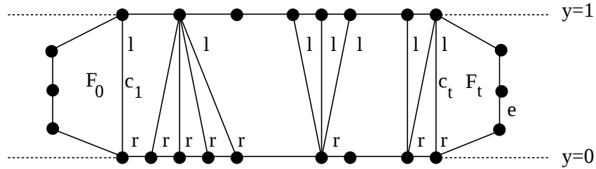
Figure 12: Outerplanar graph G .
