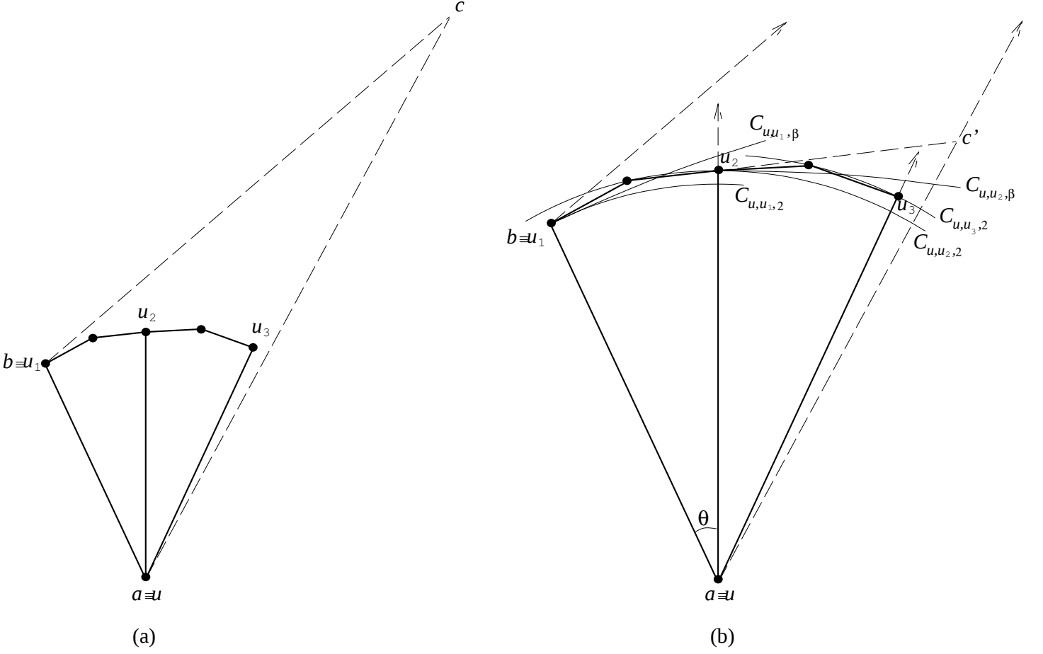
Figure 2: (a) Fan F_u \beta -drawn inside \triangle abc , and (b) details on how to \beta -draw F_u .
