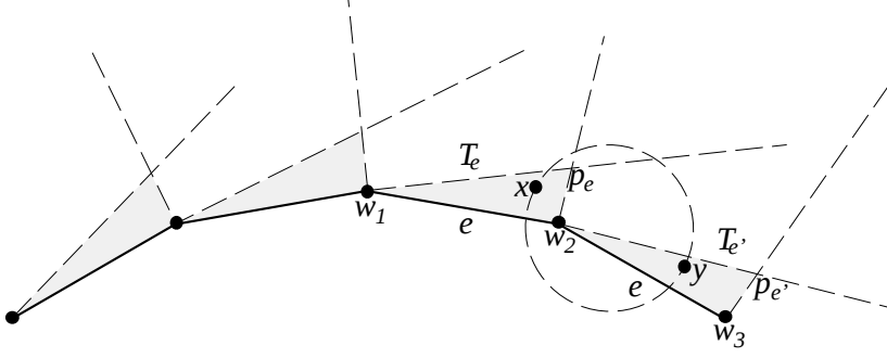
Figure 3: Illustration for the proof of Theorem 3.1
