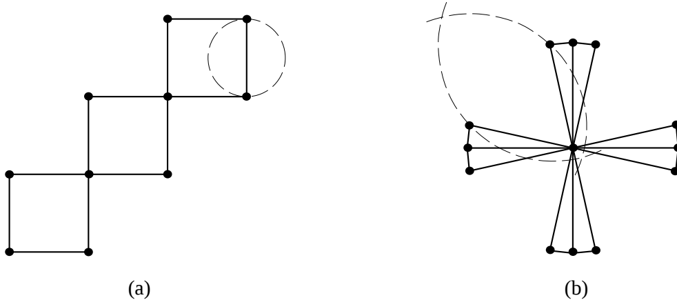
Figure 1: (a) A Gabriel drawing, and (b) a relative neighborhood drawing.
