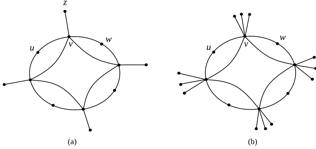
Figure 6: (a) An outerplanar graph that does not admit a [1] -drawing, and (b) an outerplanar graph that does not admit a \beta -drawing for 1 < \beta \leq 2 .
