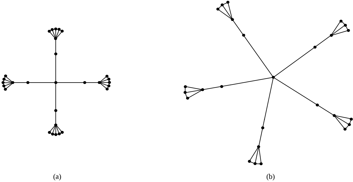
Figure 5: (a) A \beta -drawing for 1 < \beta < \frac{1}{1-\cos(\frac{2\pi}{5})} , and (b) a \beta -drawing for \frac{1}{1-\cos(\frac{2\pi}{5})} < \beta < 2 .
