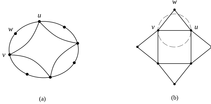
Figure 4: (a) An octagon graph G , and (b) a [1] -drawing of G .
