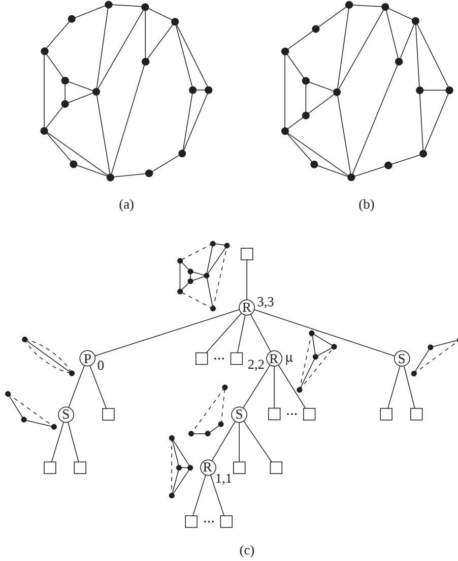
Figure 1: (a) A strictly-convex drawing of a biconnected planar graph G . (b) A convex drawing of G . (c) The SPQR-tree of G and the skeletons of its nodes. The non-trivial virtual edges are drawn with dashed lines, the trivial virtual edges are represented by solid lines, the Q-nodes are represented by squares, and the skeletons of the Q-nodes are not shown.
