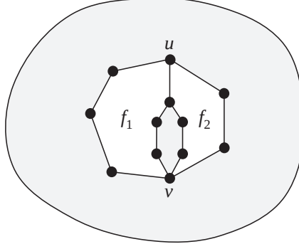
Figure 3: A split component drawn inside \Gamma .
