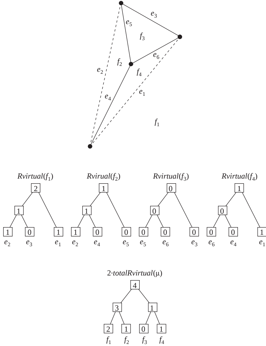
Figure 5: The skeleton of R-node \mu in Fig. 1.c, the balanced binary trees for its faces, and the balanced binary tree for \mu .
