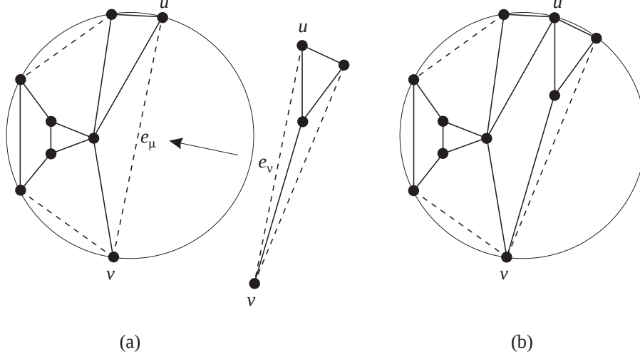
Figure 4: An example of the construction in the proof of Theorem 1.
