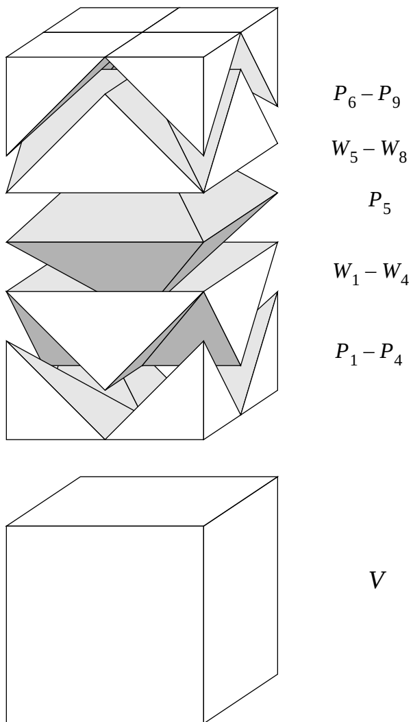
Figure 4: Partition of domain V into full or truncated instances of octahedra/tetrahedra used by the topological-separator for d = 2
