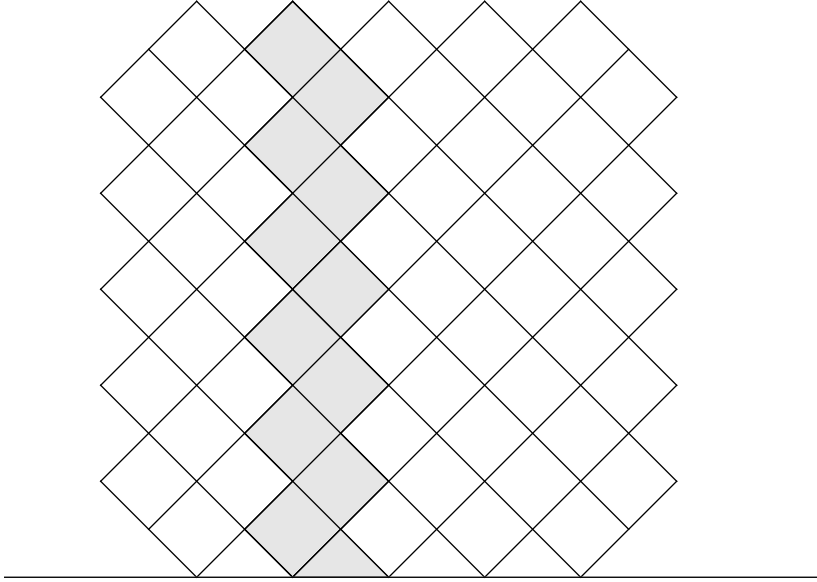
Figure 2: Zig-zag band of diamonds forming the subdomain assigned to an individual processor for d = 1
