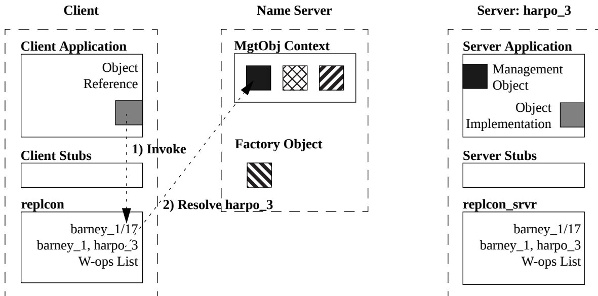
Figure 5a: Diagram of an invocation. Step 1, the client calls a method on an object reference it holds. Step 2, the replcon client class chooses harpo_3 and resolves it management object from the namespace.
