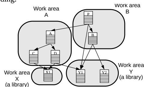
Figure 4: Software units are grouped into work areas
