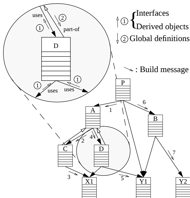
Figure 5: Propagation of the build operation.
