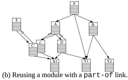
Figure 7: Reusing modules
