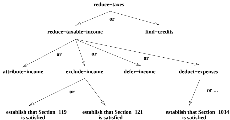
Figure 3.1: Part of the plan hierarchy.
