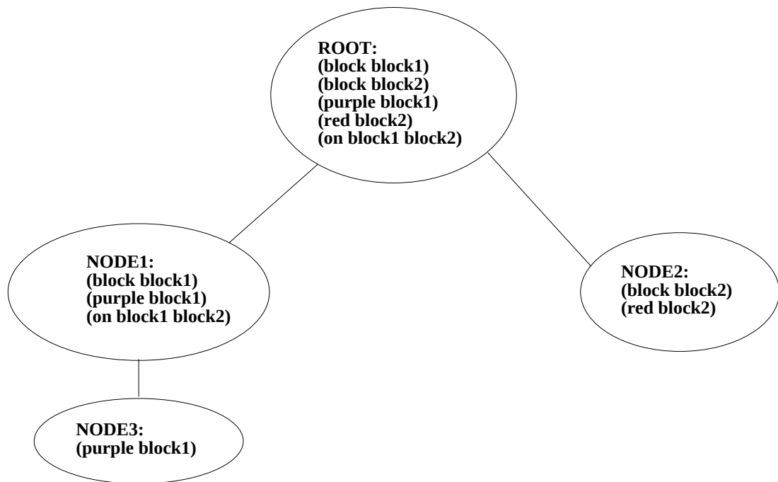
Figure 4.2: A case lattice with more facts.
