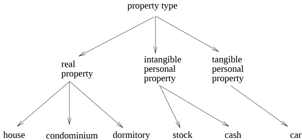
Figure 3.4: Part of the property-type hierarchy.
