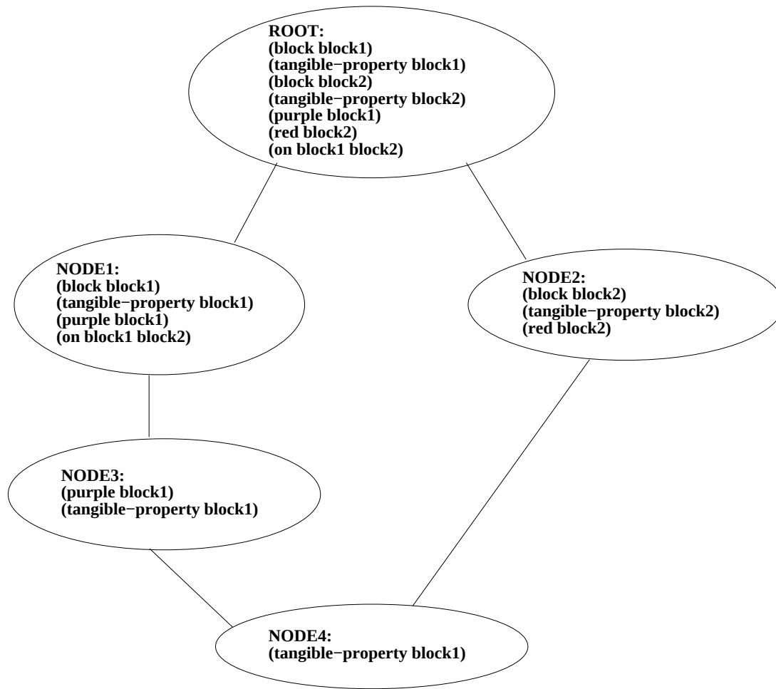
Figure 4.3: A case lattice with facts and abstractions.
