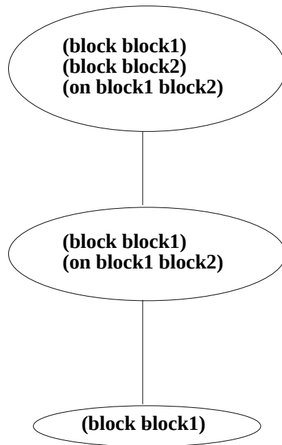
Figure 4.1: A simple case lattice.
