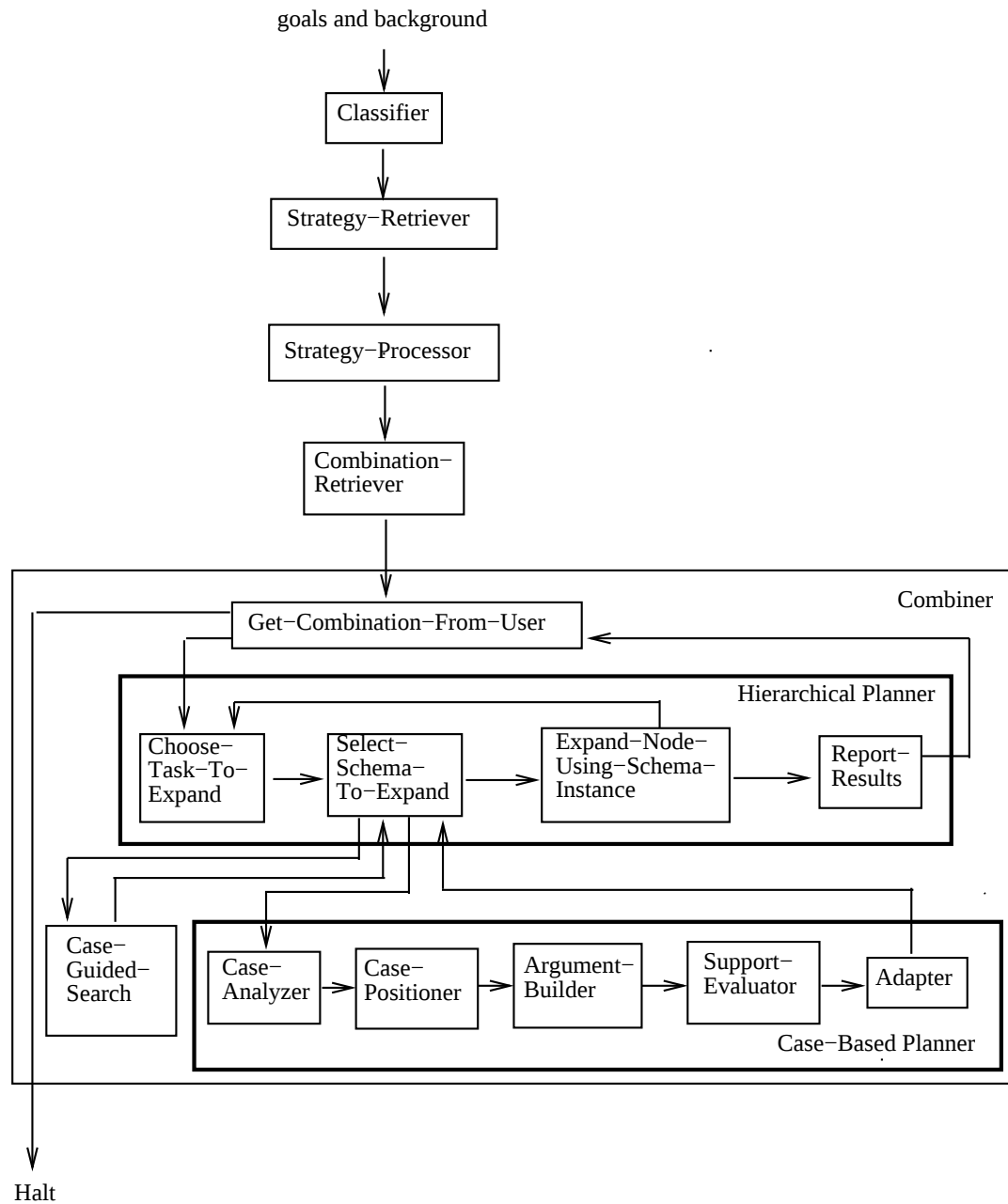
Figure 5.2: The Combiner's place in CHIRON's architecture.
