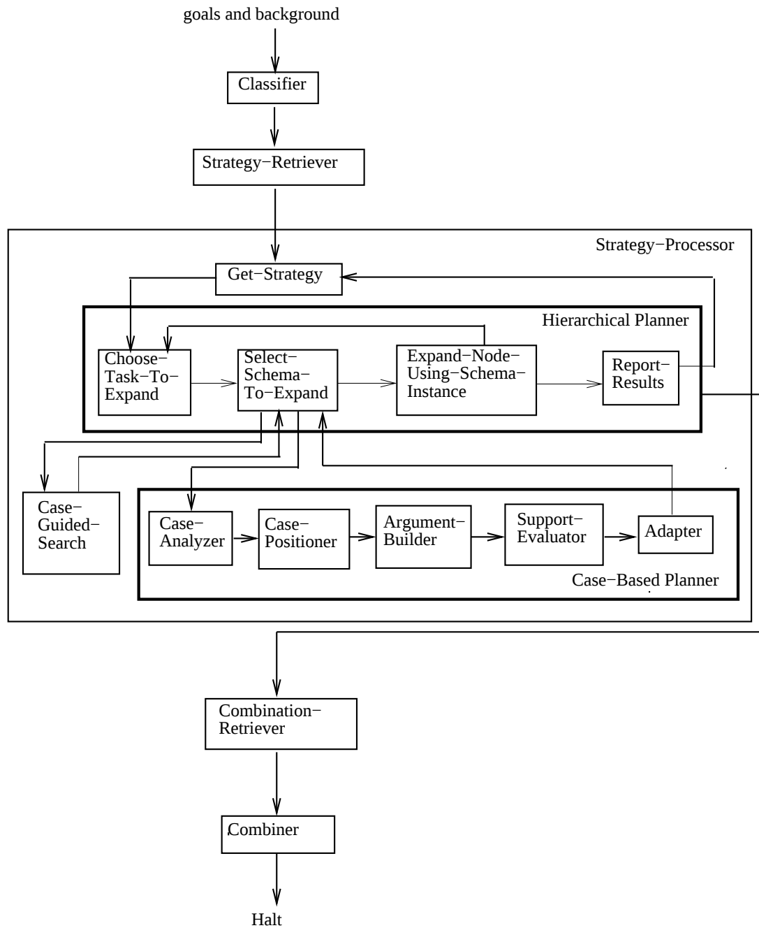
Figure 5.1: The Strategy-Processor in context
