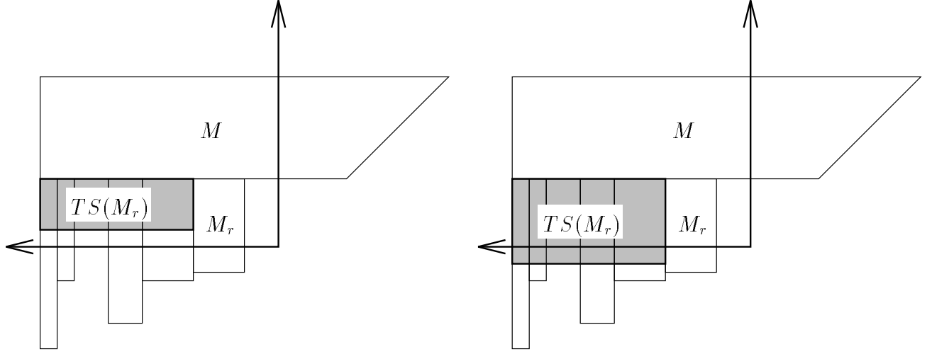
(a) In this case the entire TS(M_r) structure lies above the bottom of the query region, implying that we can individually examine all Type IV right siblings of M_r .
