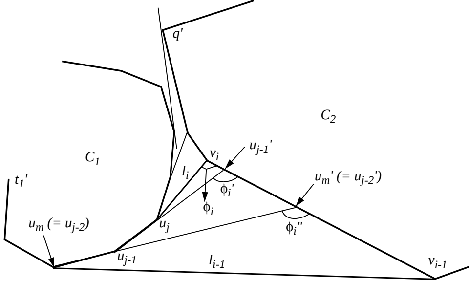
Figure 11: Lemma 9
