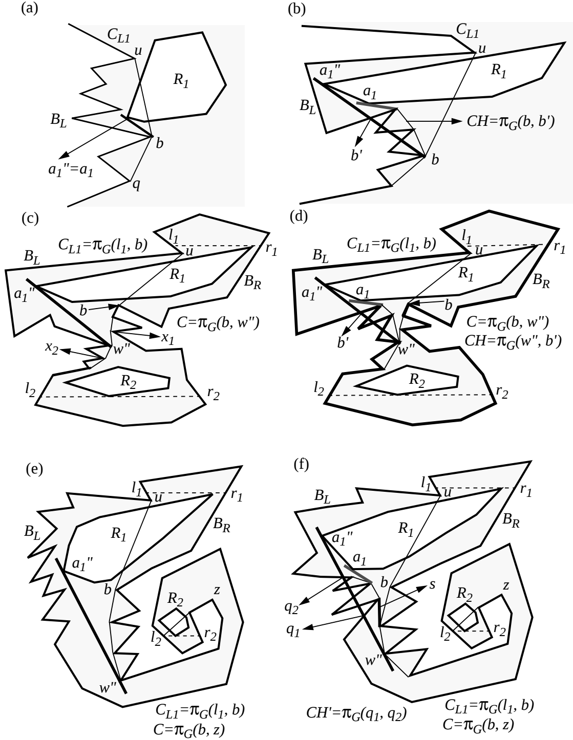
Figure 7: Steps 5(b)i–5(b)ii of Algorithm Pseudo-Hourglass and proof of Lemma 4: (a) b \in B_L and (b, a_1'') \cap (B_L - \{b\}) = \emptyset ; (b) b \in B_L and (b, a_1'') \cap (B_L - \{b\}) \neq \emptyset ; (c) b \in B_R, w'' \in B_L and (w'', a_1'') \cap (B_L - \{w''\}) = \emptyset ; (d) b \in B_R, w'' \in B_L and (w'', a_1'') \cap (B_L - \{w''\}) \neq \emptyset ; (e) b \in B_R, w'' \in B_R and (w'', a_1'') \cap B_L = \emptyset ; and (f) b \in B_R, w'' \in B_R and (w'', a_1'') \cap B_L \neq \emptyset .
