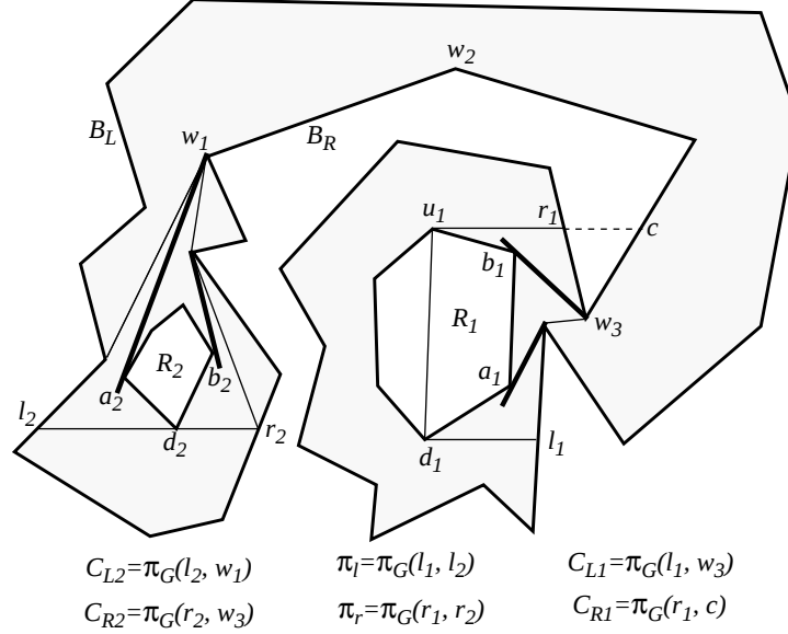
Figure 4: Step 4 of Algorithm Pseudo-Hourglass and proof of Lemma 4. As for step 4, notice how we get the bounding convex chains C_{L1}, C_{R1}, C_{L2} and C_{R2} , especially C_{R1} and C_{R2} ; as for Lemma 4, note that R_1 and R_2 do not intersect any of the bounding convex chains, S_1 = (u_1, r_1) \cup (u_1, d_1) \cup (d_1, l_1) , S_2 = (l_2, r_2) , and H_G = (a_1, b_1) \cup (a_2, b_2) \cup \pi_G(a_1, a_2) \cup \pi_G(b_1, b_2) is properly contained in S_1 \cup S_2 \cup \pi_l \cup \pi_r .
