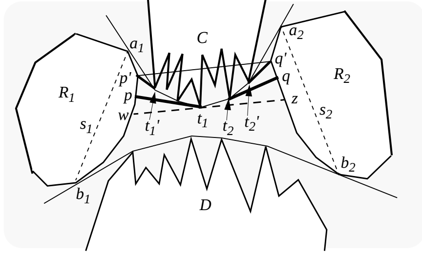
Figure 8: Lemma 6
