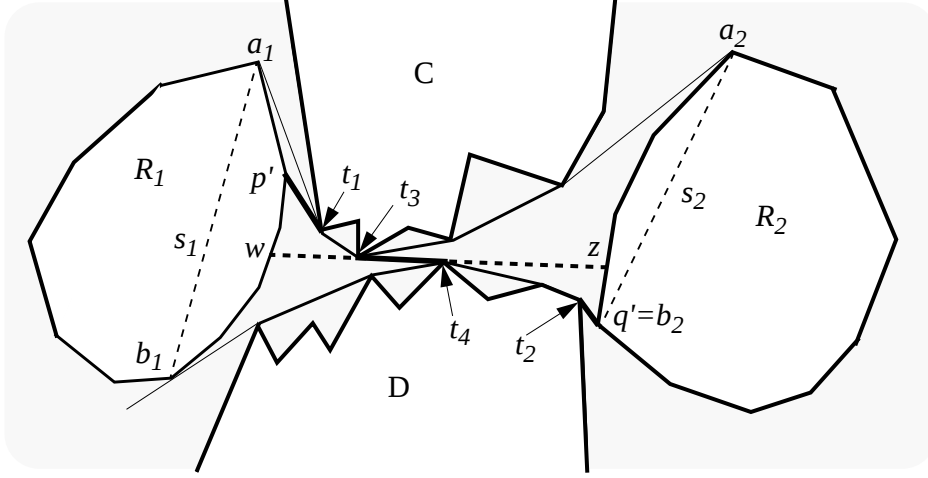
Figure 9: Lemma 7
