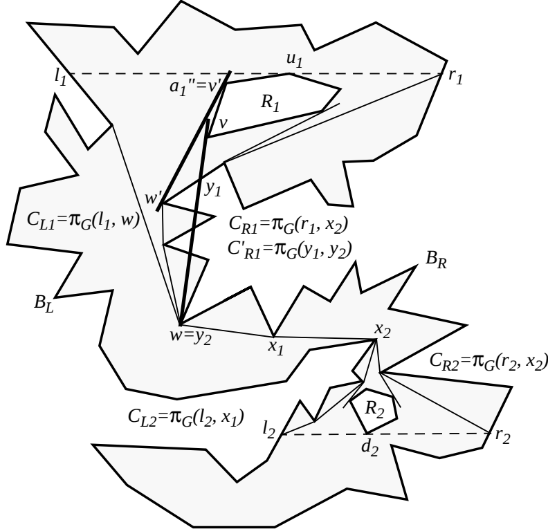
Figure 3: A running example for Algorithm Pseudo-Hourglass in the case where \pi has no cusps and C_{L1} \cap R_1 = \emptyset .
