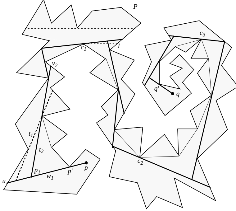
Figure 15: Computing \pi_L(p, q) by Algorithm Prelim : the window w_2 following w_1 is chosen to be t_2 since it extends farther than t_1 , and so on.
