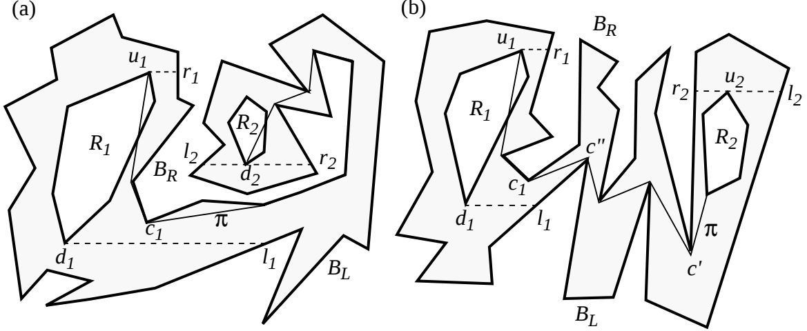
Figure 5: Step 3(b)iiA of Algorithm Pseudo-Hourglass and proof of Lemma 2: r_1 and l_1 are obtained by projecting u_1 and d_1 horizontally to the right; r_1 is on B_R and l_1 is on B_L .
