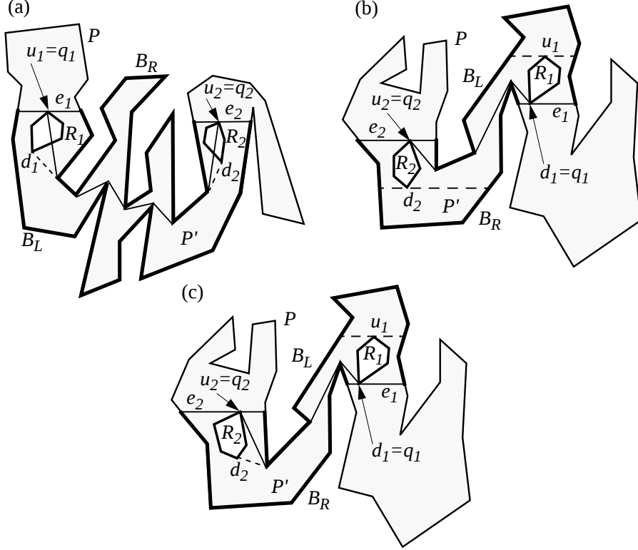
Figure 1: Left and right boundaries B_L and B_R of P : (a) several choices of (q_1, q_2) satisfy condition (ii) but only one satisfies (i); (b) several choices of (q_1, q_2) satisfy condition (i) (e.g., (u_1, d_2) is also valid) but only one satisfies (ii); (c) neither (i) nor (ii) alone enforces a unique choice of (q_1, q_2) , but their conjunction does.
