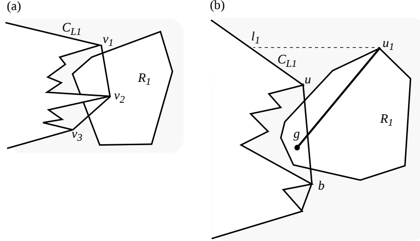
Figure 6: Proof of Lemma 3: (a) impossibility for C_{L1} to have more than one edge intersecting R_1 ; (b) finding edge (u, b) .
