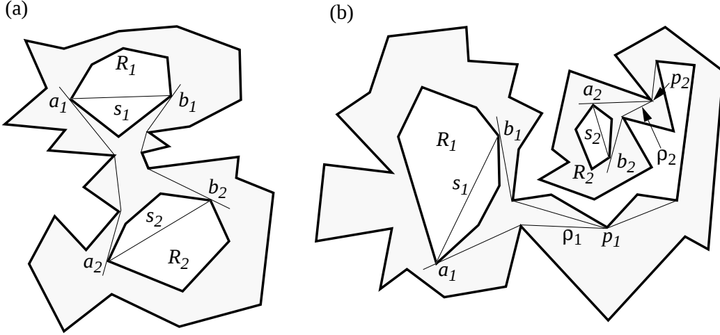
Figure 2: Geodesic hourglass H_G and geodesic external tangents: (a) H_G is open; (b) H_G is closed.
