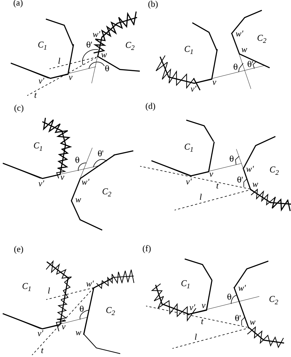
Figure 14: The cases (a)–(f) in step 2 of Algorithm Double-Search .
