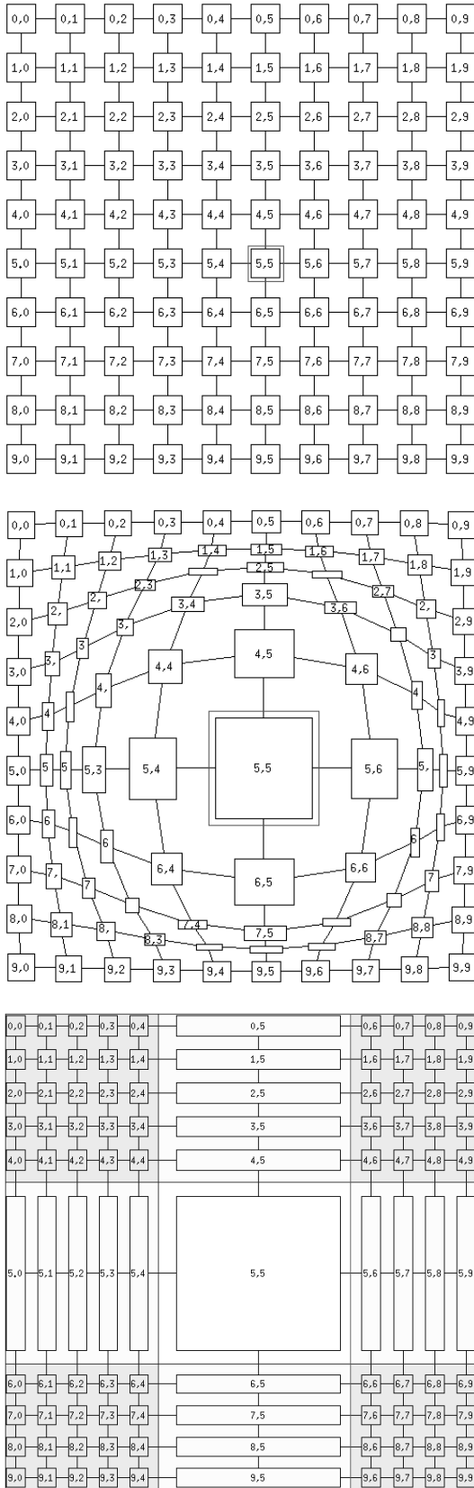
Figure 8: A symmetric layout, its view stretched with a rectangle handle and its view stretched with four bar handles. Orthogonal stretching can stretch to any degree without destroying order and symmetry.
