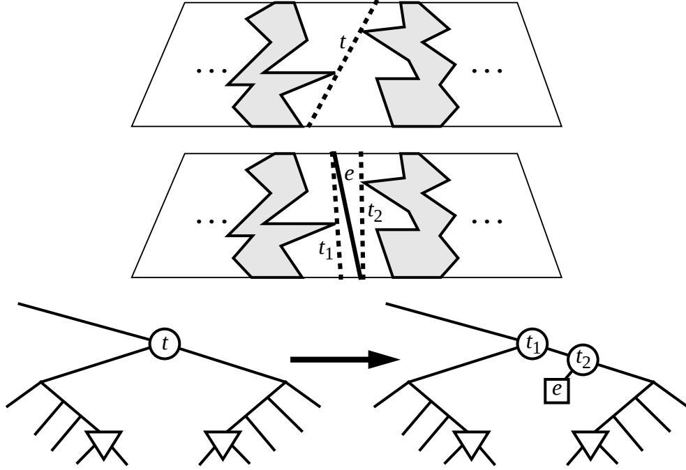
Figure 2.13: Update of the trapezoid tree caused by parting a monotone path in the normalization structure because of an edge insertion.
