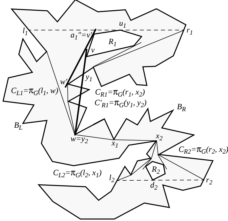
Figure 3.3: A running example for Algorithm Pseudo-Hourglass in the case where \pi has no cusps and C_{L1} \cap R_1 = \emptyset .
