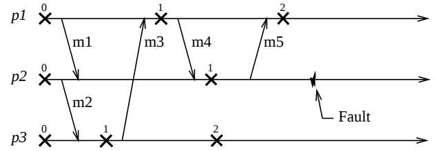
Figure 1. Domino effect when recovering from a fault. The “x”s indicate checkpoints. To recover, all processes must be rolled back to their initial checkpoints.
