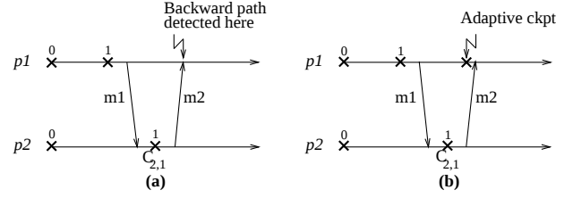
Figure 3. (a) zigzag cycle (involving C_{2,1} ) is detected at receipt of m2 , (b) an adaptive checkpoint is taken to prevent the cycle from forming, so the sender's checkpoint ( C_{2,1} ) is useful.
