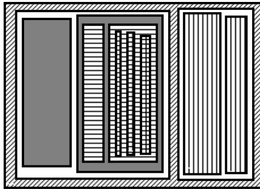
Figure 7: TreeViz Treemap
