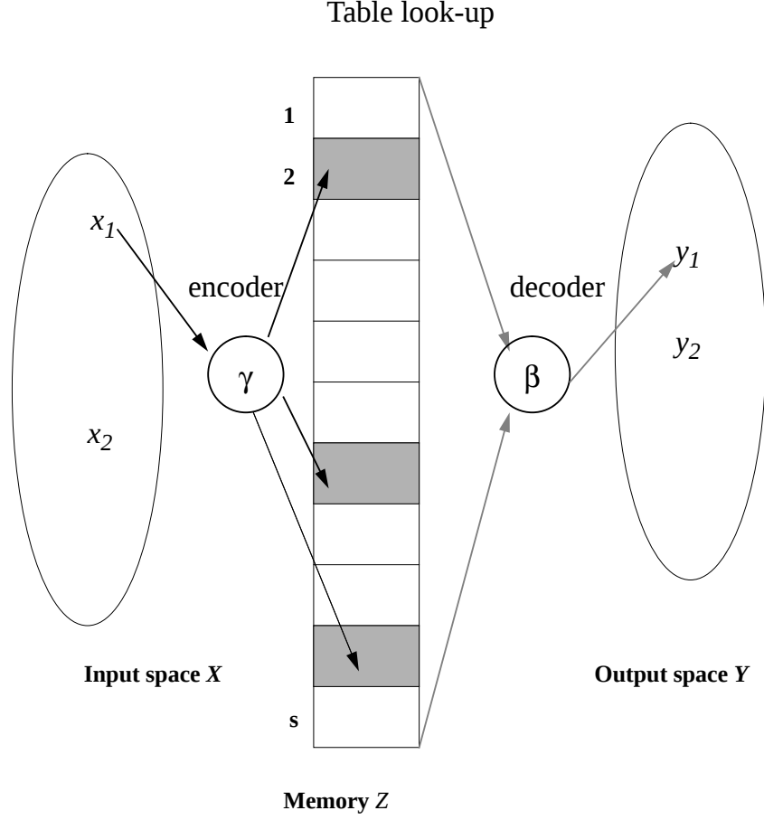
Figure 1: An example memory-based learning system. The encoder \gamma maps an input from the input space X into a set of addresses and the decoder \beta maps the set of activated memory locations into an output in the output space Y .
