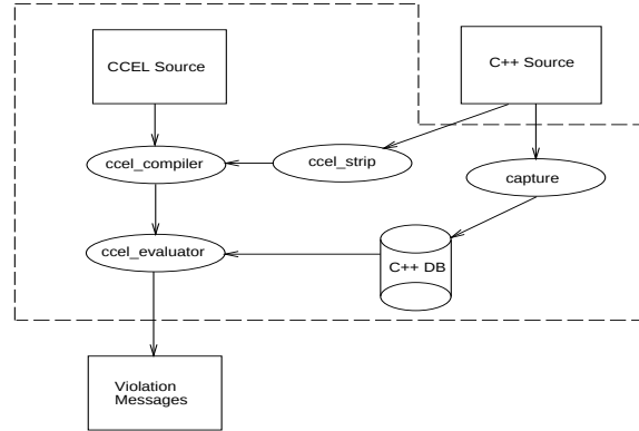
Figure 2: Clean++ Architecture
