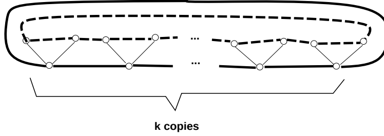
Figure 6: An example showing that the performance bounds of the algorithms in Theorems 1.1 and 1.2 are existentially tight.
