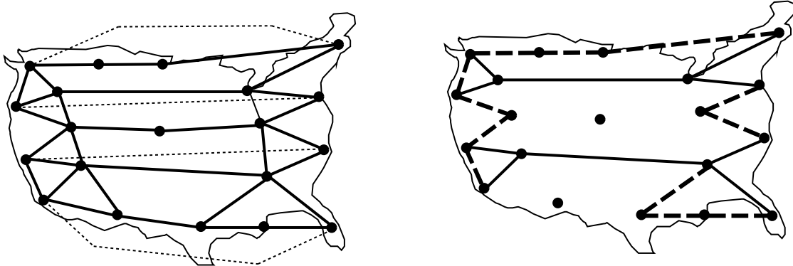
Figure 1: An instance of the unweighted generalized two-connected Steiner network problem and an optimum solution. Solid edges correspond to unit-cost links; dotted edges connect site pairs. In the right figure, the solid edges correspond to first phase one-connecting solution. The thick dashes form an augmentation to two-connect the solid trees.
