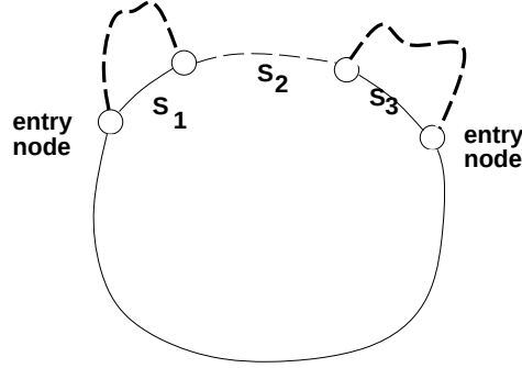
Figure 4: A segment S is said to be forbidden if the endpoints of S are entry nodes, and S consists of three subsegments S_1S_2S_3 , where S_2 is a nonskeletal segment, the endpoints of S_1 form a short-cut, and the endpoints of S_3 form a short-cut. The dark dashed paths represent paths in G(t) - C between the endpoints of S_1 and between the endpoints of S_3 .
