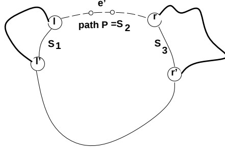
Figure 5: Lemma 5.13: e' is some nonskeletal edge in C , and P is the maximal nonskeletal path containing e' in C . Let l and r be the endpoints of P , and let their corresponding entry nodes be l' and r' . Then the segment \langle e'l', r' \rangle is a forbidden segment for e' . The dark lines show paths in G(t) - C between each of l and r and the entry nodes l' and r' corresponding to them.
