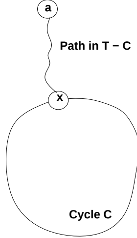
Figure 2: A node x in the cycle C is called an entry node if it is reachable in T - C from an active node a .
