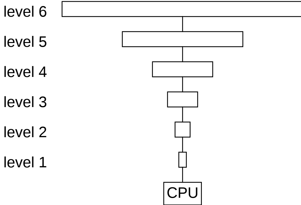
Figure 1: The HMM hierarchical memory model [1].
