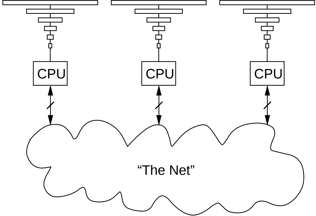
Figure 2: A parallel hierarchical memory. The P individual memory hierarchies can be either of type HMM or of type BT. The P CPUs can communicate among one another via the network; we assume, for example, that the P records stored in their accumulators can be sorted in O(\log P) time.
