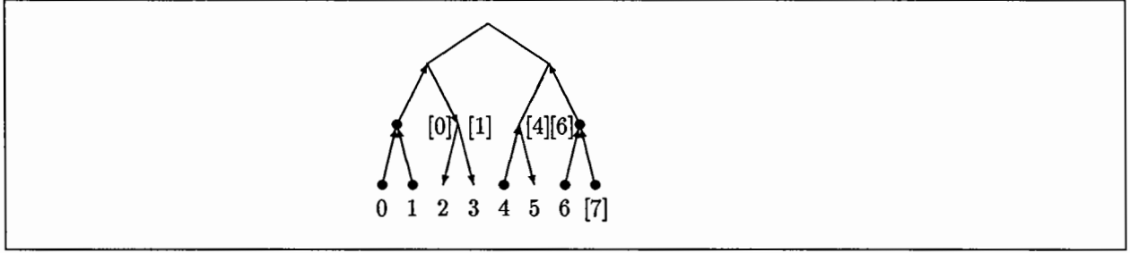
Figure 3: Processor traversal of the progress tree.
