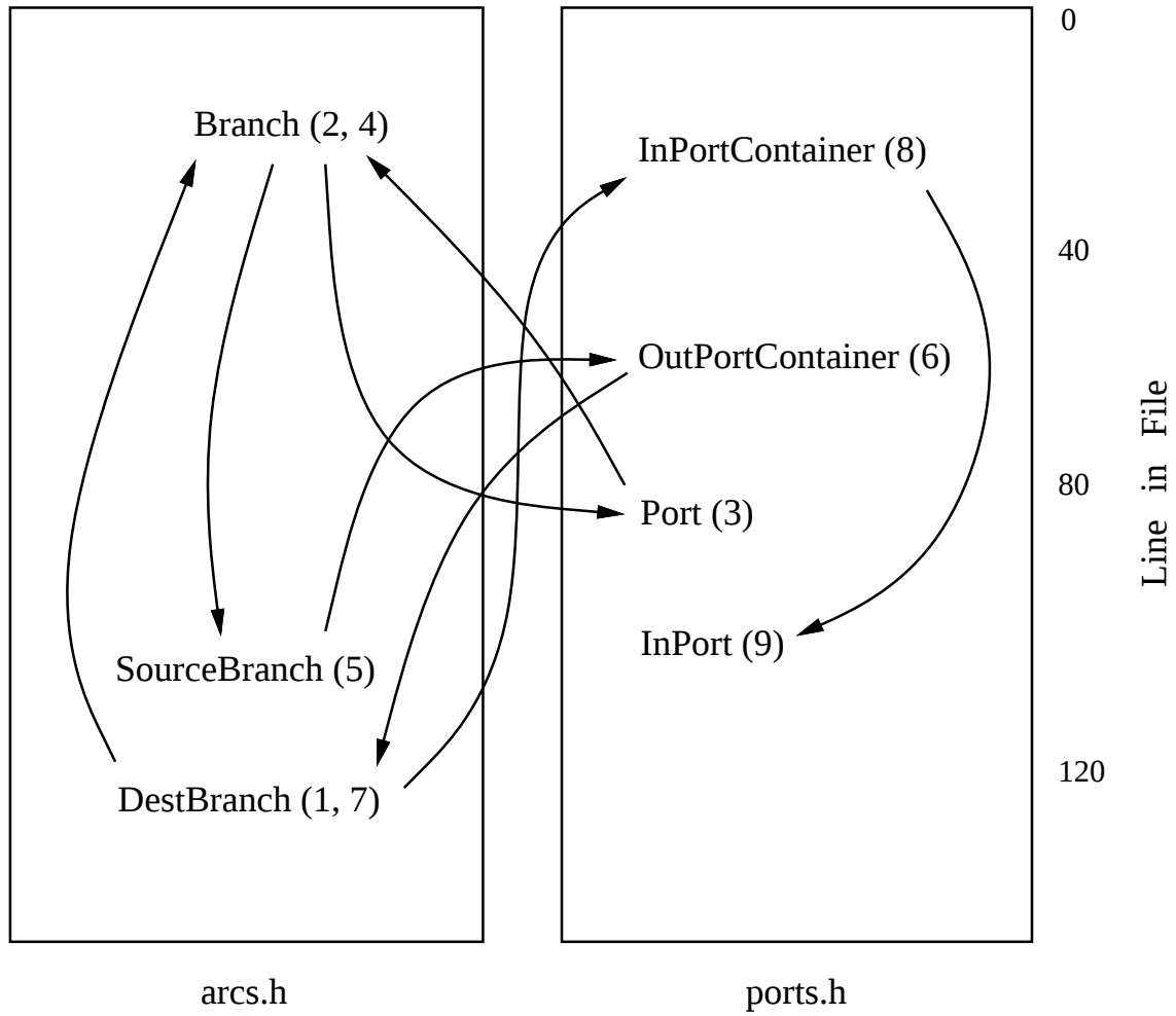
Figure 1: Route taken by programmer search for body of putToken .
