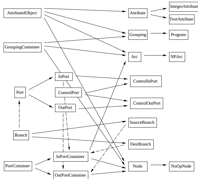
Figure 2: Part of a real inheritance graph. Arrows run from superclasses to subclasses. Broken arrows indicate some of the “uses” relations present in the classes pictured.
