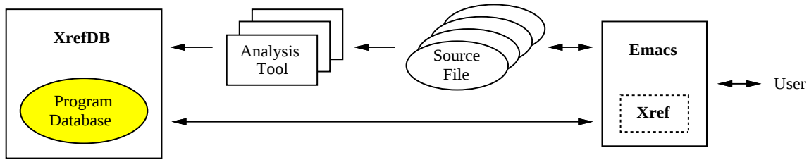
Figure 3: The architecture of XREF/XREFDB.
