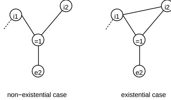
FIG. 5.3. Network additions for the statement (\text{role } i_2 \text{ slot } i_1) .
