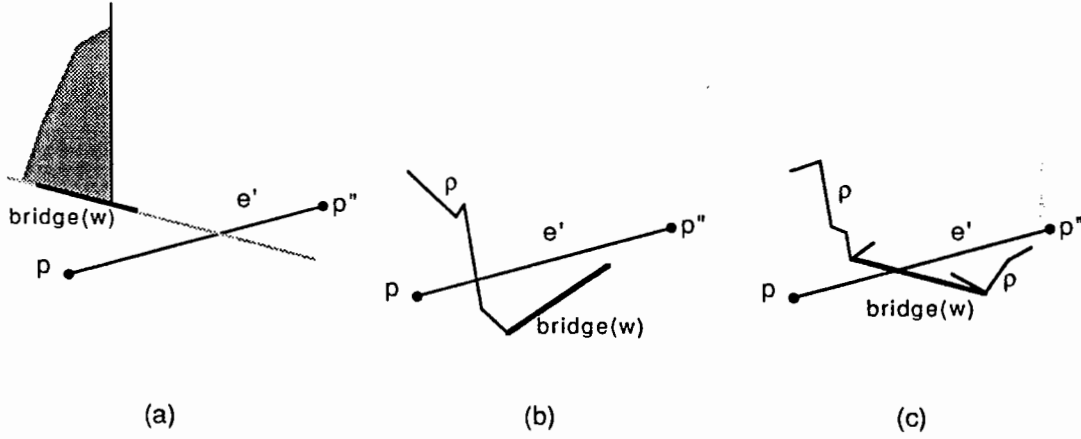
Figure 2: The different cases in the recursive search for the first intersection between edge segment e' and the silhouette \rho .
