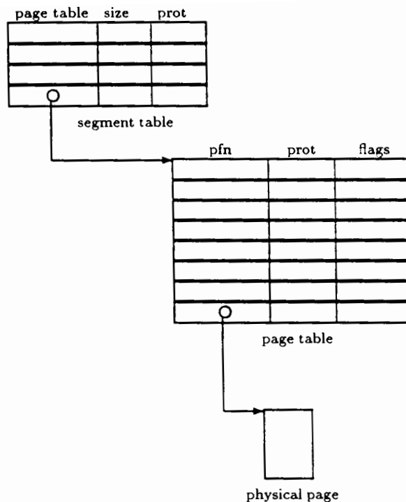
Figure 10: Virtual memory data structures – default pmap
