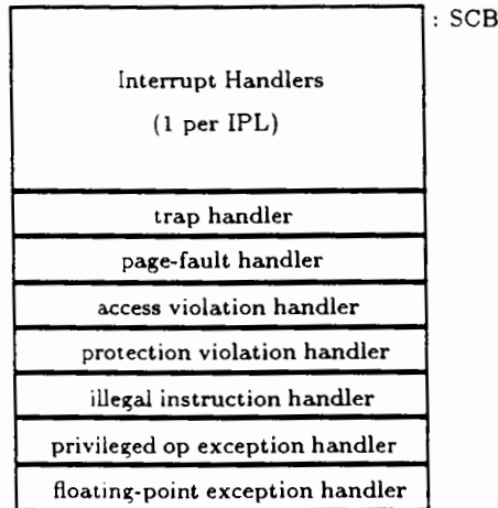
Figure 1: System Control Block
