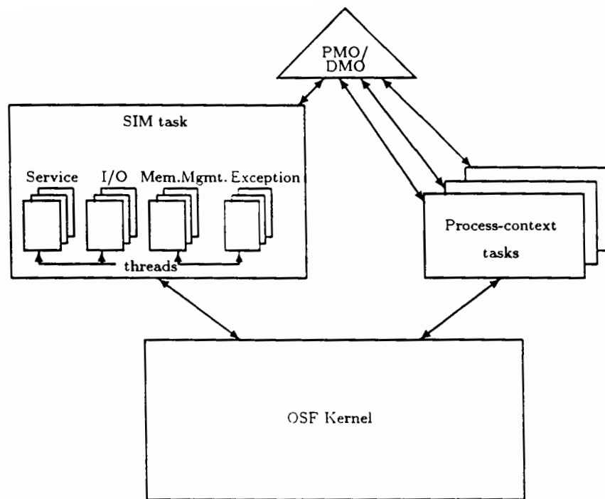
Figure 2: OSF/1-based simulator architecture
