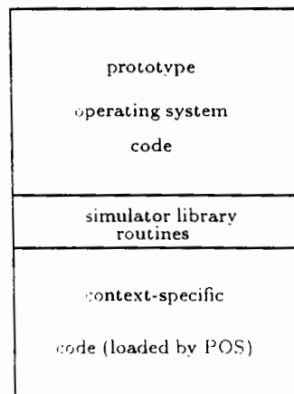
Figure 4: Code that runs within a process-context task
