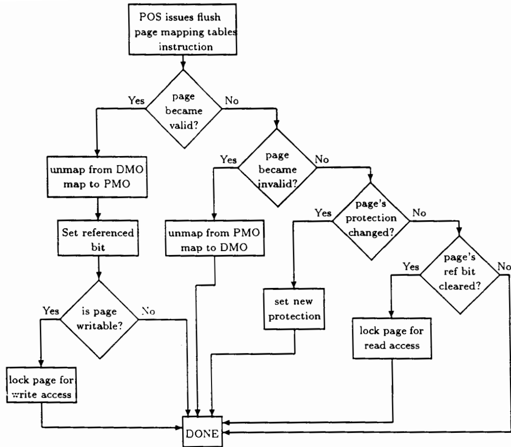
Figure 8: Flush Operation
