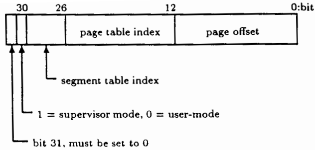
Figure 9: Virtual address format – default pmap
