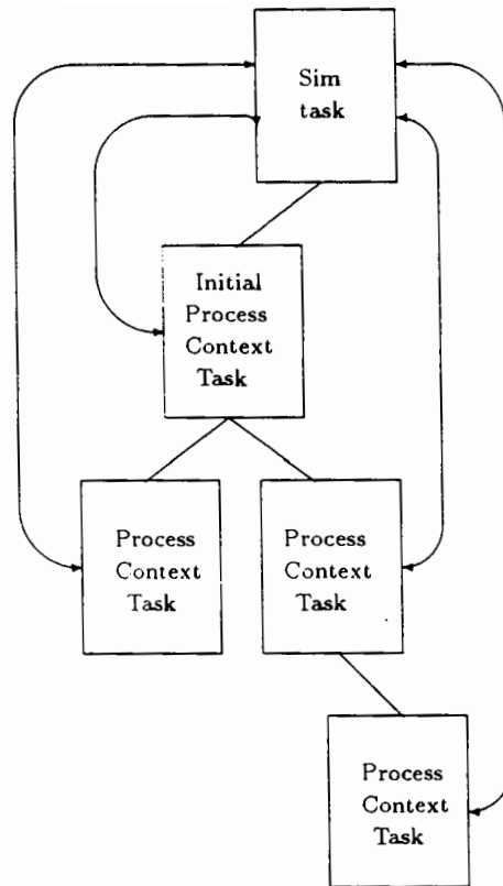
Figure 3: Simulator task hierarchy
