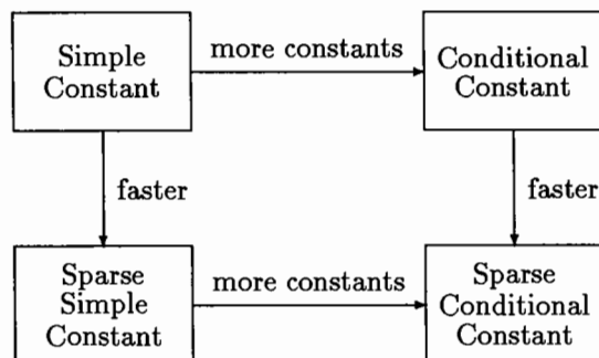
Figure 5. Relationship among the four constant propagation algorithms.
