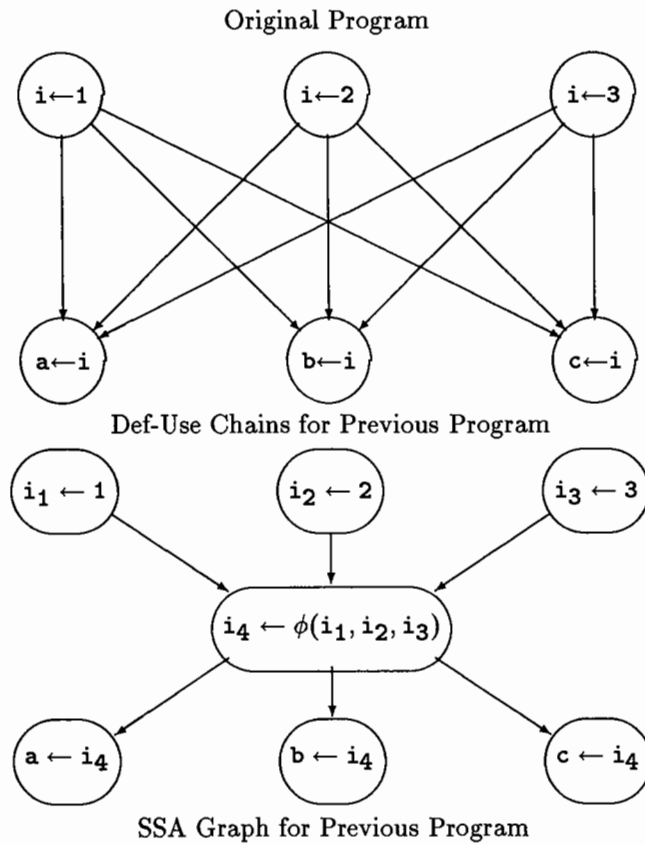
Figure 12. Worst-case behavior of def-use chains.
