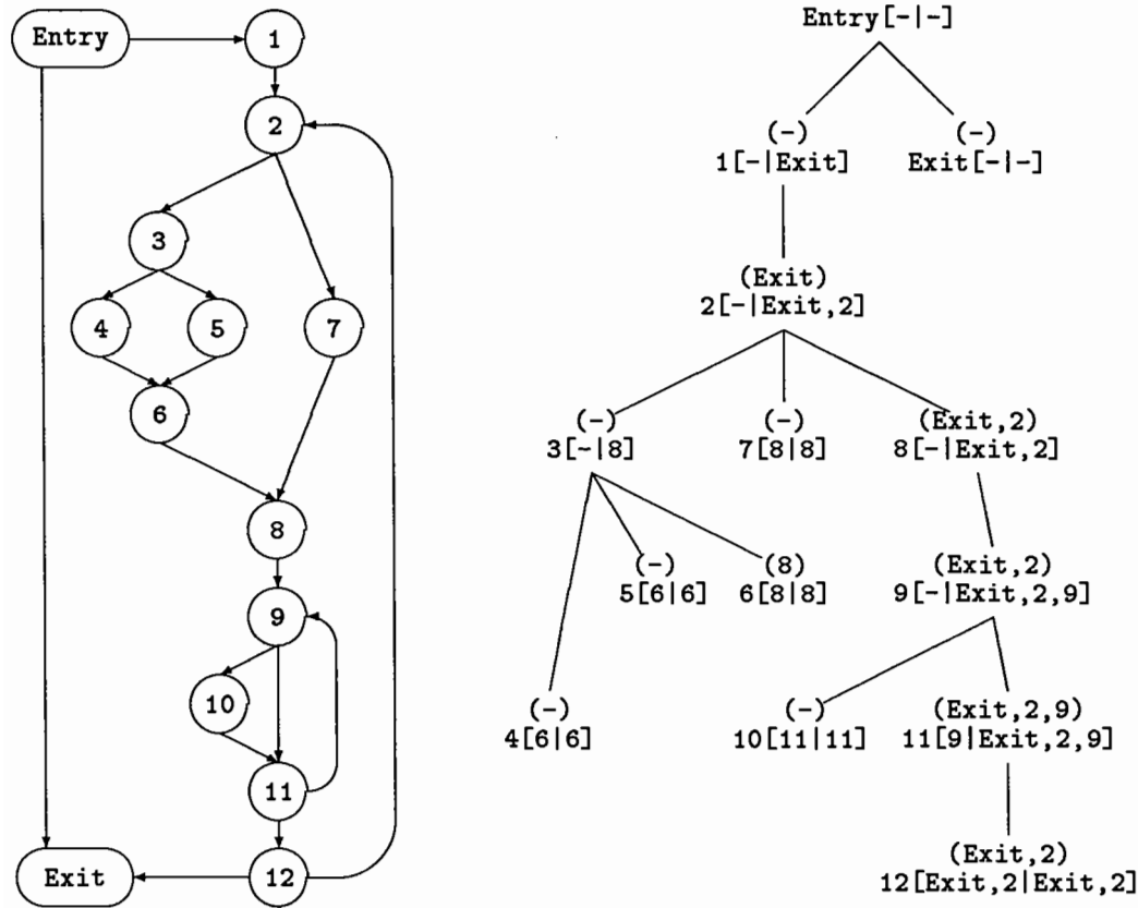
Figure 9. Control flow graph and dominator tree of the simple program.
