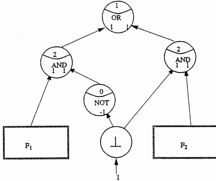
Figure 5: Neural net architecture for F_1 \cup F_2 . Note that the constant 1 can be implemented as x + \bar{x} .
