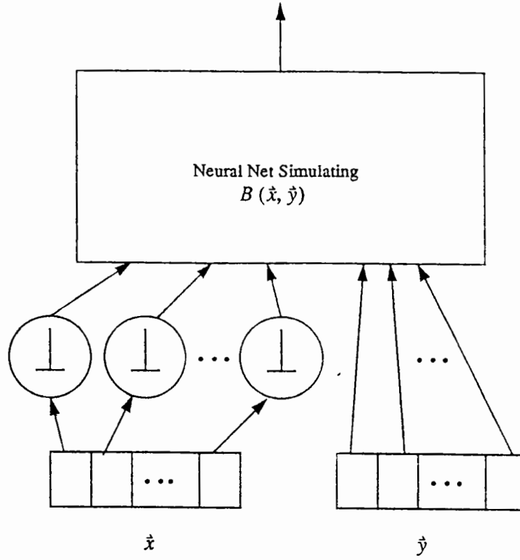
Figure 4: Net architecture for the NET MEMBERSHIP problem.
