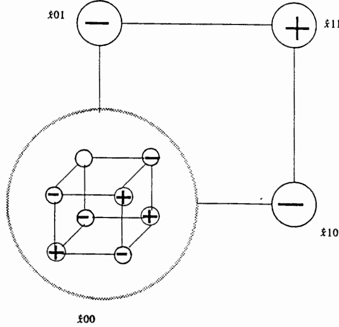
Figure 2: Examples used to show that 2-CASCADE NEURAL NET TRAINING is \mathcal{NP} -complete.
