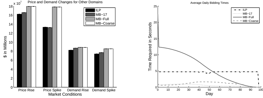
Fig. 1.6. (a) Revenue from deliveries in extreme market conditions. (b) Average daily bidder times in Price Rise conditions. Other market conditions had similar run times.
