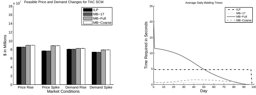
Fig. 1.5. (a) Revenue from deliveries under feasible SCM market conditions. (b) Average daily bidder times in Price Rise conditions. Other market conditions had similar run times.
