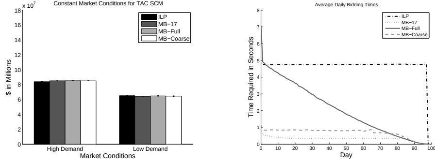
Fig. 1.4. (a) Revenue from deliveries under constant market conditions. (b) Average daily bidder times in high demand conditions. Low demand bidder times were similar.
