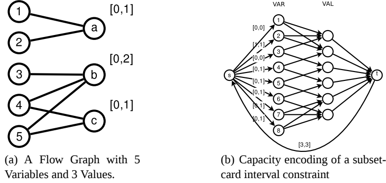
Fig. 1. Flow graphs for the open-GCC constraint
