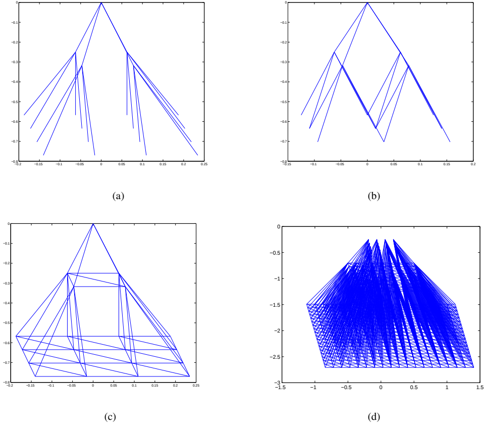
Figure 2: (a) A three-level pyramid graph with no overlap between adjacent receptive fields, (b) a three-level pyramid graph with an overlap of one, (c) a three-level pyramid graph with no overlap and intra-level edges and (d) a generalized pyramid graph with three levels, multiple roots, an overlap of one and intra-level edges in levels one and two.
