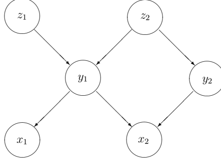
Figure 6: A fragment of a pyramid graph used to illustrate the process of learning state spaces and conditional probability tables.
