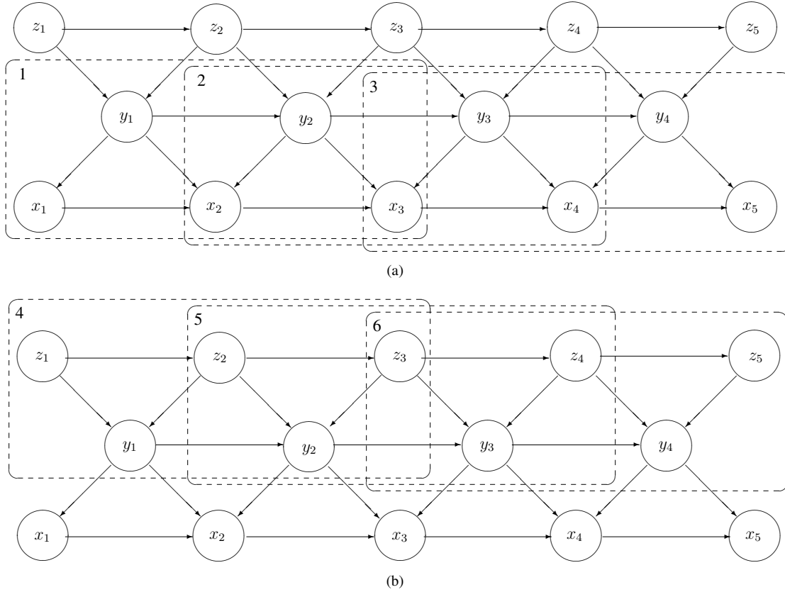
Figure 3: A fragment of a three-level PBN showing (a) the decomposition of the first layer into three separate parameter estimation problems and (b) an analogous decomposition of the second layer.
