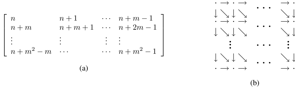
Figure 1: One level in a pyramid graph illustrating (a) the pyramid-graph node-numbering scheme and (b) the pattern of intra-level connections (if present) showing how this pattern together with the node-numbering scheme ensure that the graph is acyclic; the width of a level is m = w + (p - 1)(w - o) where w is the width of the receptive fields, p is the width of the parent level and o is the overlap between adjacent receptive fields.
