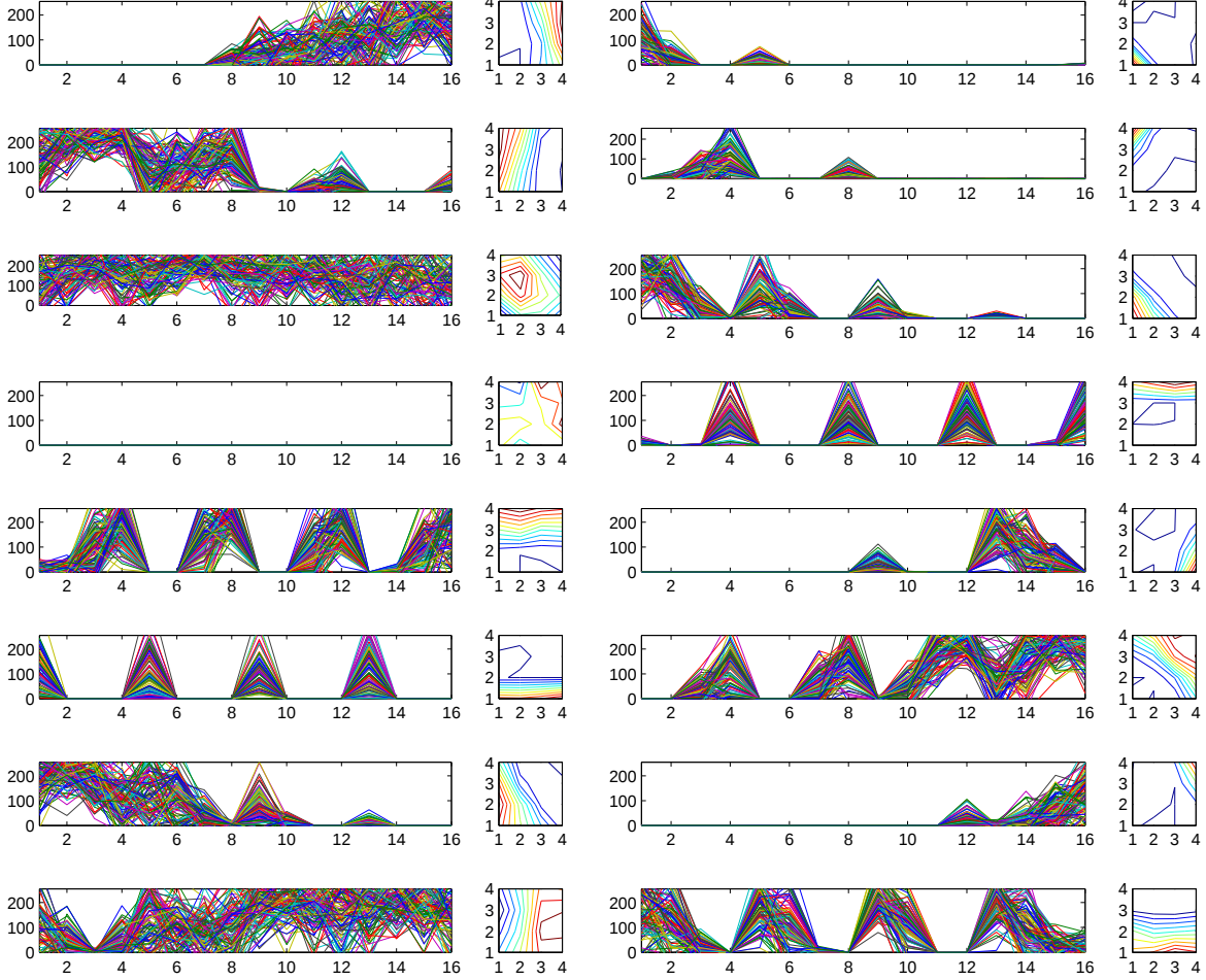
Figure 5: Two visualizations of the mixture-of-Gaussians classifier learned from the MNIST data set.
