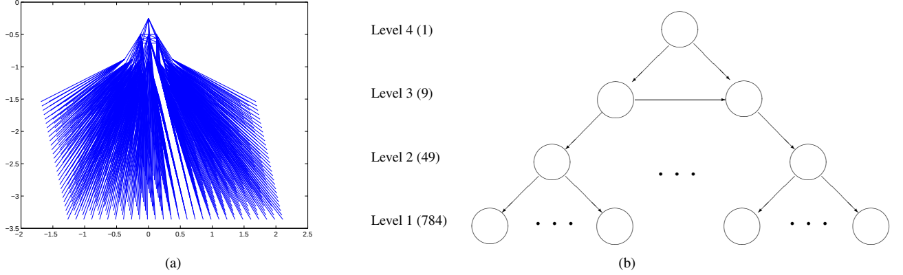
Figure 4: The four-level PBN used in the experiments with MNIST data set.
