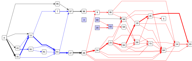
Figure 8: The Precedence Graph Projected wrt Machine 3 after the Relaxation of 3 \rightarrow 68 .
