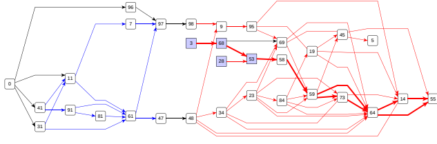
Figure 7: The Precedence Graph Projected wrt Machine 3 with some Critical Arcs from Machine 5.
