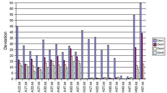
Figure 12: Visualizing the Effect of Multiple Relaxations (set B)
