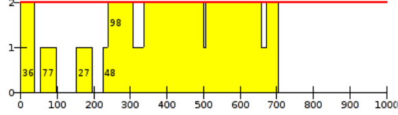
Figure 5: The Profile of Machine 3 after the First Call to RELAX.
