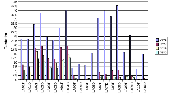
Figure 11: Visualizing the Effect of Multiple Relaxations (set A)
