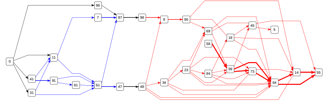
Figure 6: Projection of Precedence Graph wrt Machine 3
