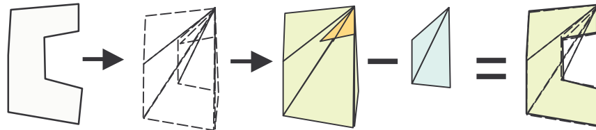
Figure 3. A signed area triangle fan covering a non-convex region.
