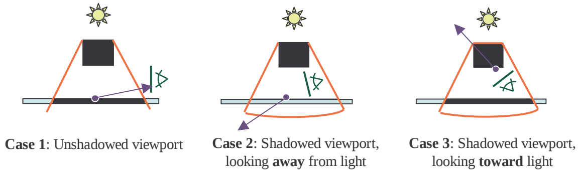
Figure 4. Three cases distinguished by our algorithm.
