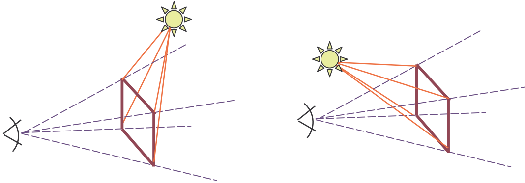
Figure 2: The viewport occlusion pyramid (solid red) extends from the light source to the viewport. Compare to the view frustum (dashed blue). As shown on the right, the occlusion pyramid may also be behind the viewport.
