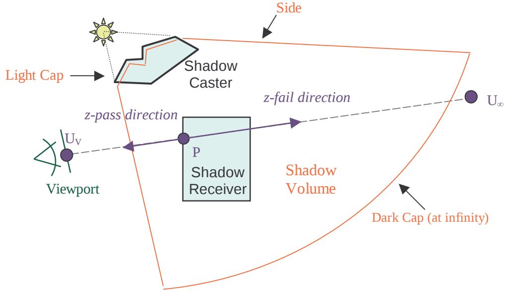
Figure 1. A 2D diagram showing shadow volume geometry
