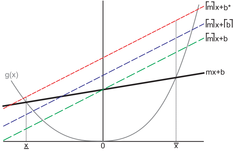
Fig. 1. Why \lceil m \rceil x + \lceil b \rceil is not a Safe Linear Overestimator.
