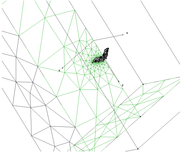
Figure 2: A Gridgen screengrab. Here, a user specifies which surfaces should be triangulated.
