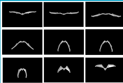
Above, shots of a wing beat taken at every 6th frame demonstrate the significant amount of deformation which occurs to the model's wings during flight.
