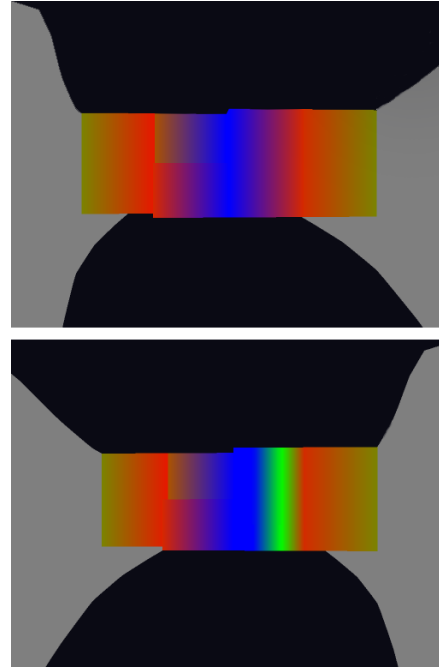
Figure 4: Here we see a cross-sectional cut of flow through a nozzle visualized at different levels of spectral order. The top image uses only a second order representation while the bottom image was generated with a 3rd order representation. At this higher level of detail the boundary layer between jet and near-wall downstream flow is resolved.
