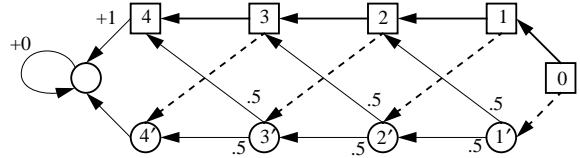
Figure 1: Simple policy iteration requires an exponential number of iterations to generate an optimal solution to the family of MDPs illustrated here (after (Melekopoglu and Condon, 1990)).
