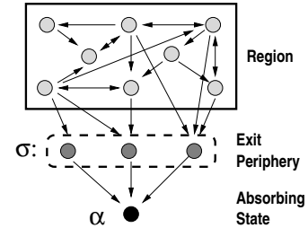
Figure 4: A Local MDP for Macro Generation
