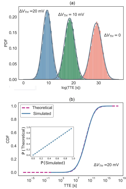
Fig. 6. (a) Statistical TTE histograms of subthreshold CMOS latches extracted by STTACC for V_{DD} = 180 mV, T = 100^\circ\text{C} , and threshold mismatch \Delta V_{TH} = 0, 10 , and 20 mV, together with the corresponding log-normal fits using the histogram mean and variance. (b) TTE CDF of a subthreshold CMOS latch extracted by STTACC vs. theoretical log-normal distribution from the mean and variance of the TTE histogram ( V_{DD} = 180 mV, T = 100^\circ\text{C} , \Delta V_{TH} = 20 mV). Inset shows the P-P plot for comparing the simulation results and the theoretical fit.
