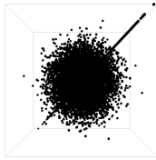
Figure 5: 2D rendering of a line in 3D space intersecting noisy sphere. AKA “skewered meatball.”
