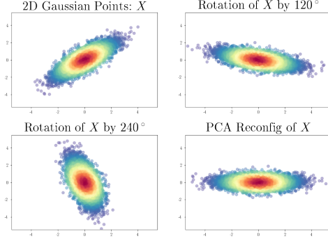
Figure 4: Left: 2D zero-mean Gaussian with covariance \begin{pmatrix} 1 & 0.8 \\ 0.8 & 1 \end{pmatrix} . We rotate X by 120^\circ and 240^\circ , respectively. Right: Points after applying PCA reorientation.
