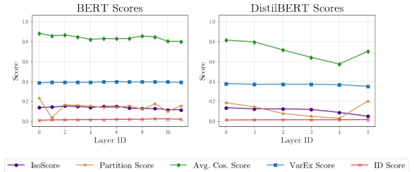
Figure 9: The 5 scores for the 12 layers of BERT, and the 6 layers of DistilBERT
