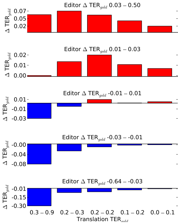
Figure 2: Effect of editing on translations of varying quality. Rows reflect bins of editors, with the worse editors (those whose changes result in increased \text{TER}_{gold} ) on the top and the most effective editors (those whose changes result in the largest reduction in \text{TER}_{gold} ) on the bottom. Bars reflect bins of translations, with the highest \text{TER}_{gold} translations on the left, and the lowest on the right. We can see from the consistently negative \Delta \text{TER}_{gold} in the bottom row that good editors are able to improve both good and bad translations.
