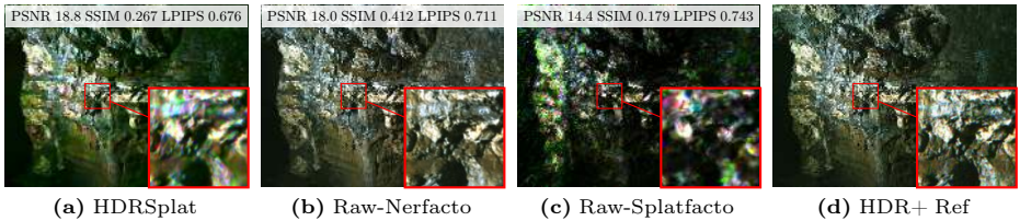
Fig. 6: Standard metrics do not measure artifacts well. HDRSplat’s render (a) is noisier throughout the image than that of Raw-Nerfacto (b), yet (a)’s PSNR is better. LPIPS varies only moderately with large visual changes, where HDRSplat is incorrectly better than Raw-Nerfacto while Splatfacto is correctly worse. SSIM better reflects the difference across (a–c).
