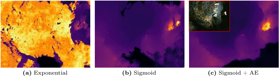
Fig. 10: Raw-Nerfacto depth maps on D8. (a) Exponential output activation causes severe geometry errors under low SNR. (b) Replacing it with a sigmoid stabilises training. (c) Adding per-image appearance embeddings (AE) further reduces residual artefacts.
