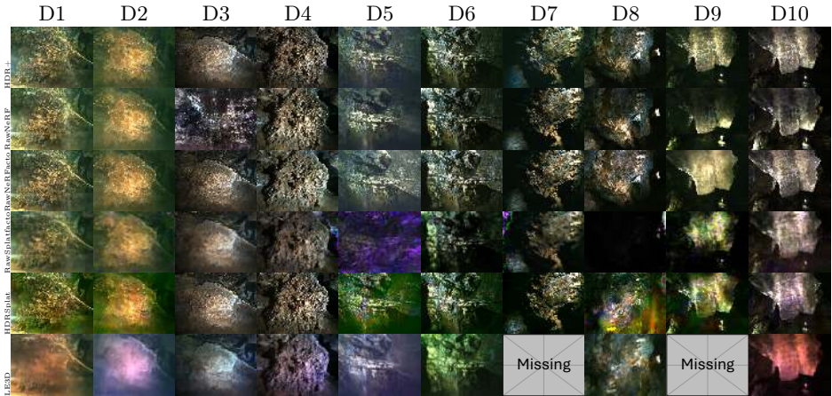
Fig. 4: Qualitative comparison of all RAW methods. Raw-Nerfacto is visibly better than its competitors, which often cannot reliably reconstruct challenging scenes.
