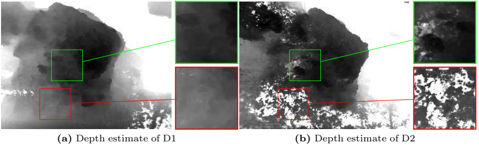
Fig. 8: Contrast loss causes floaters and gaps. Depth estimation of a) D1 and b) D2 using Raw-Nerfacto. D2 has reduced contrast due to a light appearing near the camera. This introduces floaters around the center and low-density areas.
